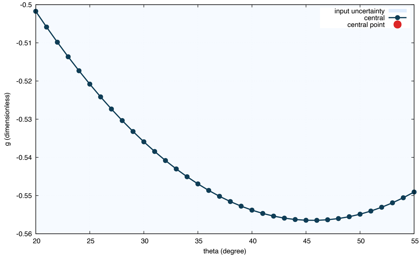
B_{s1}^{(L)} \rightarrow B_s^* \gamma ; mixing-angle sensitivity
