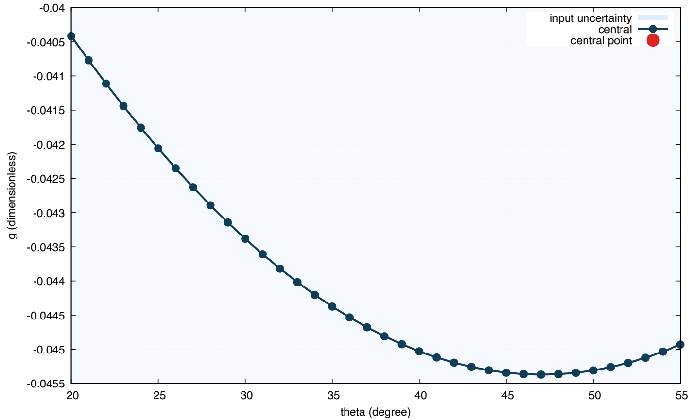
D_{s1}(2460) \rightarrow D_s^* \gamma ; mixing-angle sensitivity
