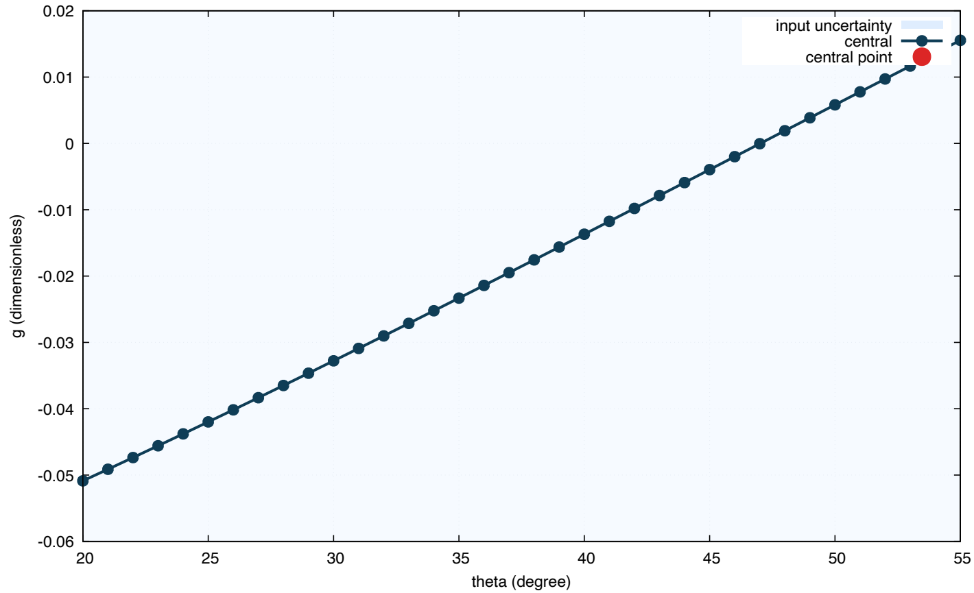
D_{s1}(2536) \rightarrow D_s^* \gamma ; mixing-angle sensitivity
