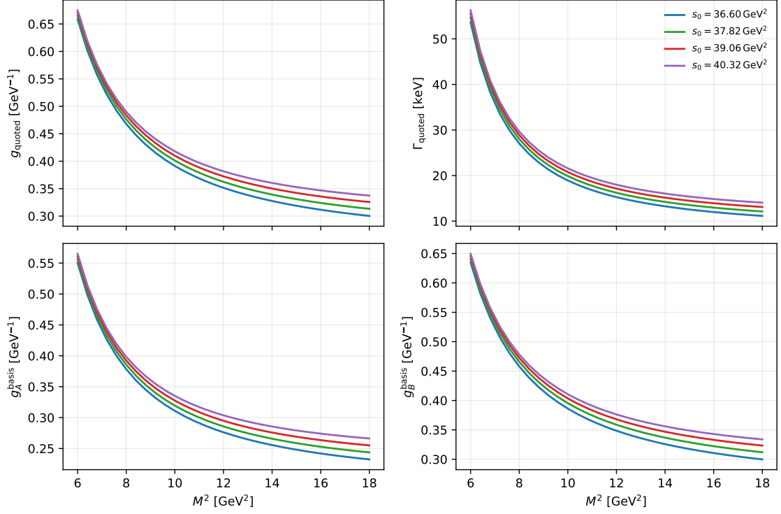
B_{s1}^{\text{low}}(5750) \rightarrow B_s \gamma stability, lattice photon normalization
