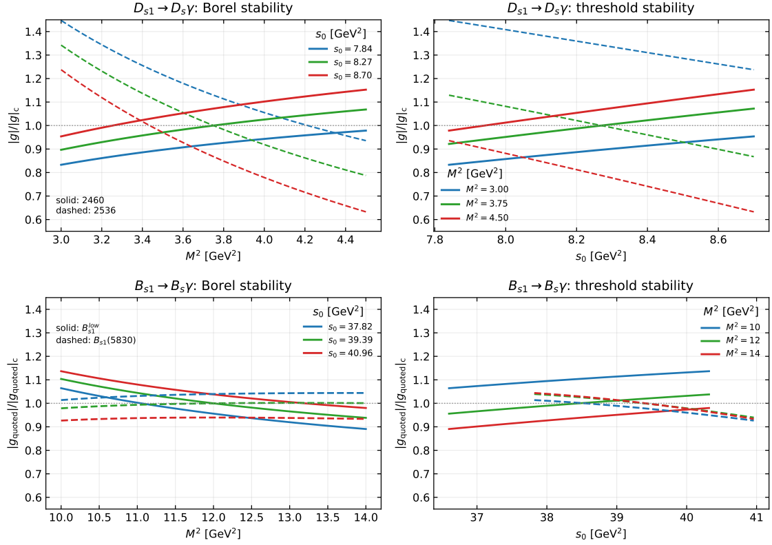
Figure 18: Selected-window stability of the physical form factors. The left column shows the M^2 dependence at selected fixed s_0 , and the right column shows the s_0 dependence at selected fixed M^2 . Solid and dashed curves denote the partner channels indicated in each panel. The D_{s1}(2536) curves show stronger relative variation because the physical amplitude is close to a cancellation point.
