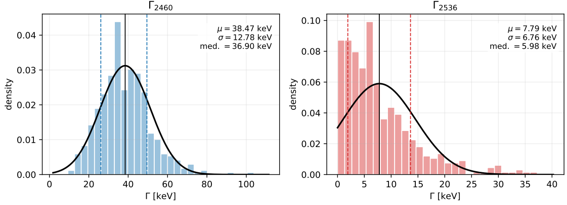
Monte Carlo width distribution, 25^\circ \leq \theta \leq 45^\circ
