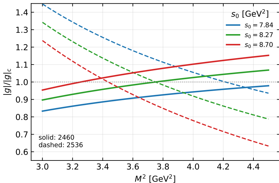
D_{s1} \rightarrow D_s \gamma : Borel stability
