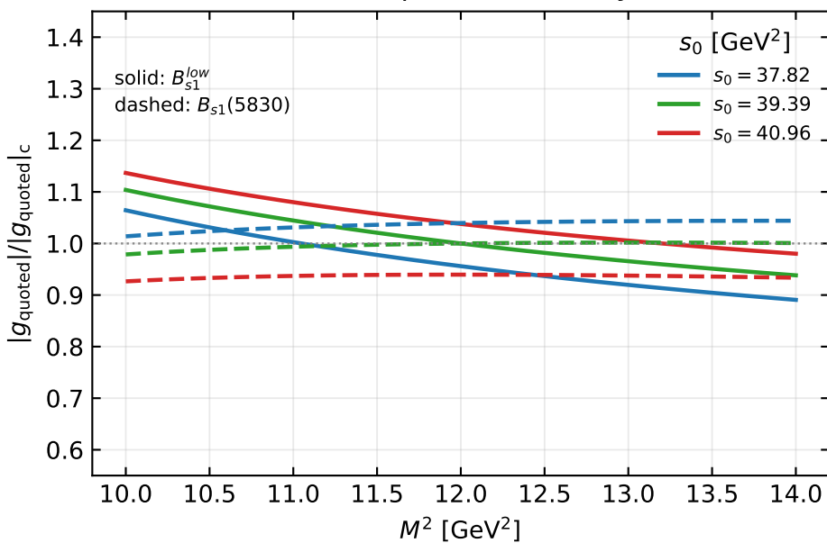
B_{s1} \rightarrow B_s \gamma : Borel stability
