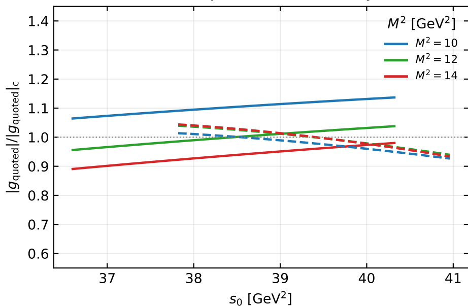
B_{s1} \rightarrow B_s \gamma : threshold stability
