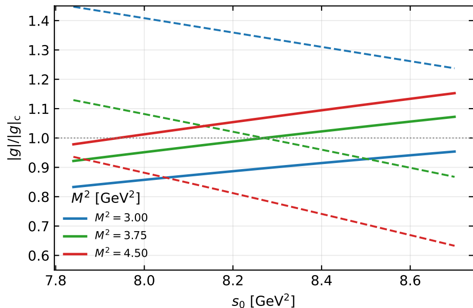
D_{s1} \rightarrow D_s \gamma : threshold stability
