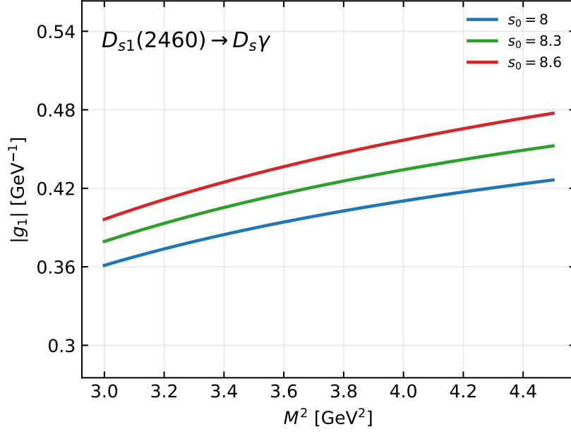
Figure 18: M^2 -dependence of the physical form factor for D_{s1}(2460) \rightarrow D_s \gamma , shown at selected fixed s_0 values. The vertical range is deliberately kept wider than the curve spread so that the visual impression reflects the actual stability of the chosen window.
