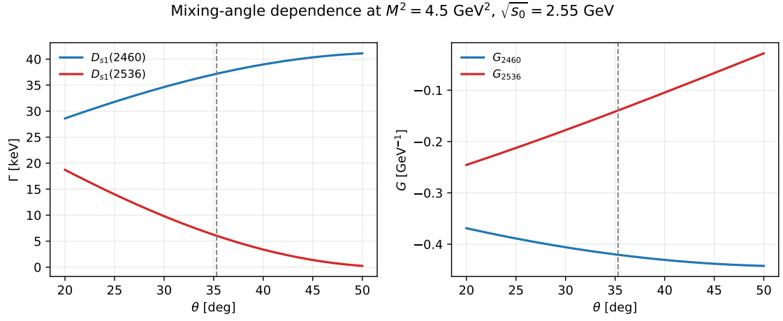
Figure 6: Mixing-angle dependence at M^2 = 4.5 \text{ GeV}^2 and \sqrt{s_0} = 2.55 \text{ GeV} . The dashed line marks \theta = 35.3^\circ .
