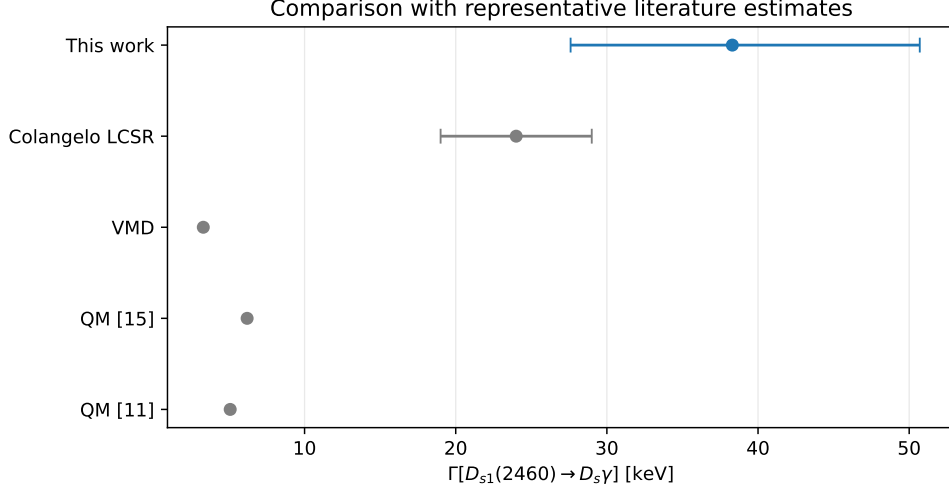
Figure 8: Comparison of the present D_{s1}(2460) \rightarrow D_s \gamma width with representative literature estimates. The Colangelo LCSR, VMD and quark-model values are from the comparison table in Colangelo, De Fazio and Ozpineci (hep-ph/0505195).
