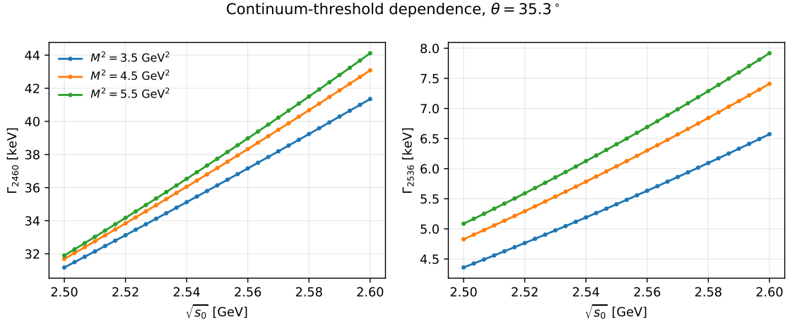
Figure 5: Continuum-threshold dependence of the matched Stage 2 widths for \theta = 35.3^\circ at three representative Borel points.
