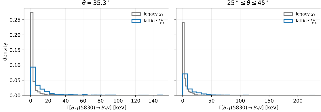
B_{s1}(5830) Monte Carlo width distributions
