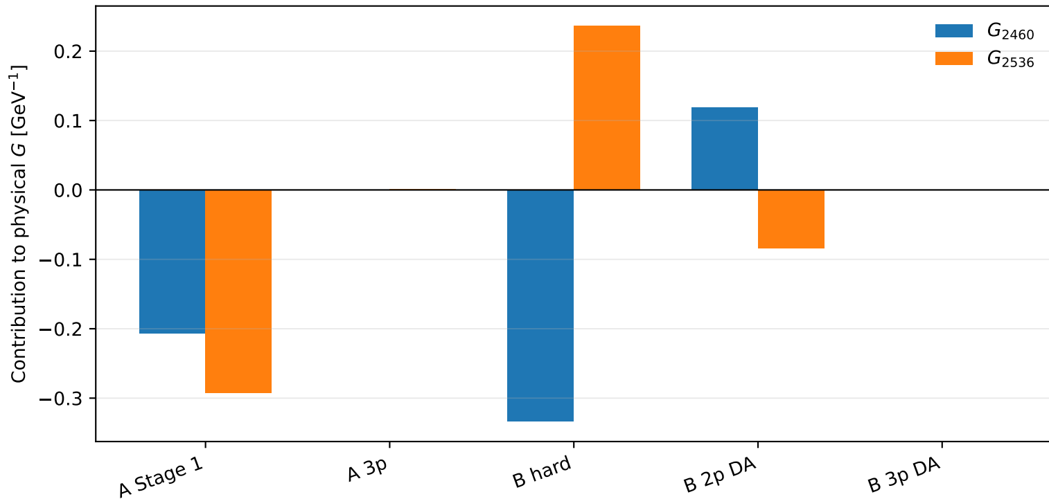
Central contribution breakdown, M^2 = 4.5 \text{ GeV}^2 , \sqrt{s_0} = 2.55 \text{ GeV}
