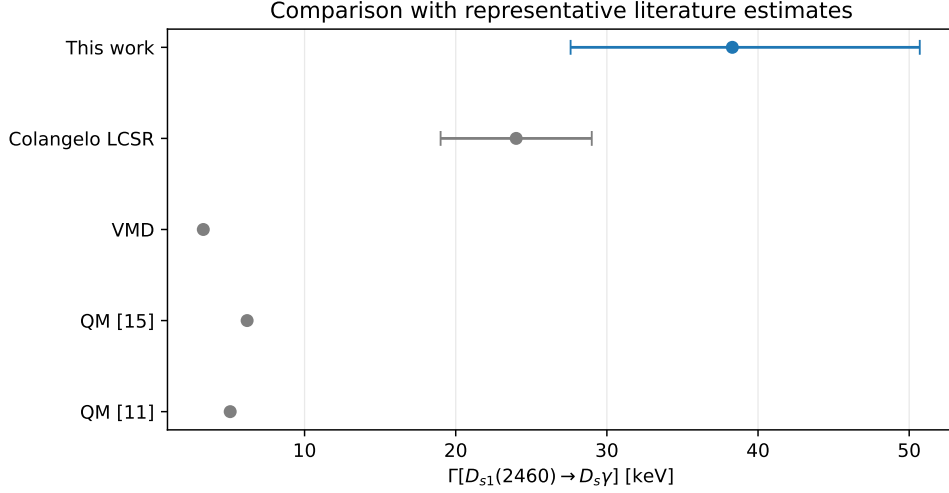
Figure 9: Comparison of the present D_{s1}(2460) \rightarrow D_s \gamma width with representative literature estimates. The Colangelo LCSR, VMD and quark-model values are from the comparison table in Colangelo, De Fazio and Ozpineci (hep-ph/0505195).
