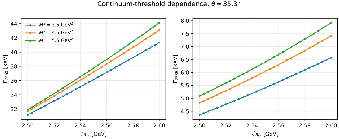
Figure 6: Continuum-threshold dependence of the matched Stage 2 widths for \theta = 35.3^\circ at three representative Borel points.
