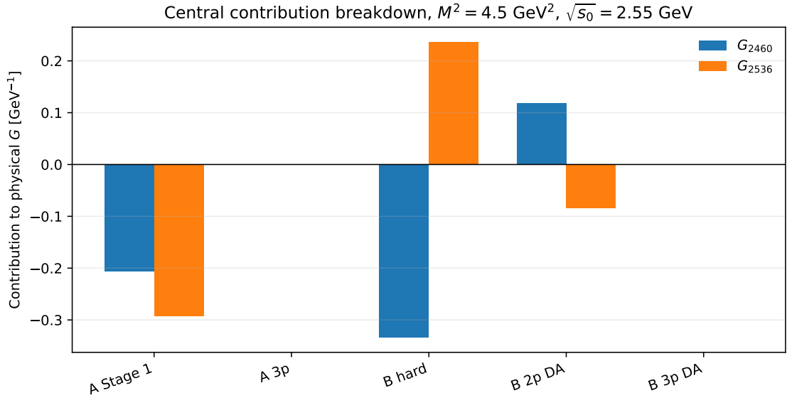
Figure 8: Contribution breakdown for the physical couplings at the central Borel and threshold point. The labels “A” and “B” refer to the axial-current and tensor-current components before physical mixing.
