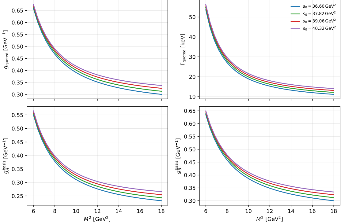
B_{s1}^{low}(5750) \rightarrow B_s \gamma stability, lattice photon normalization
