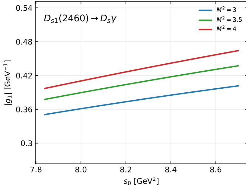
Figure 19: s_0 -dependence of the physical form factor for D_{s1}(2460) \rightarrow D_s \gamma , shown at selected fixed M^2 values. This is the complementary threshold-stability check for the same selected window.
