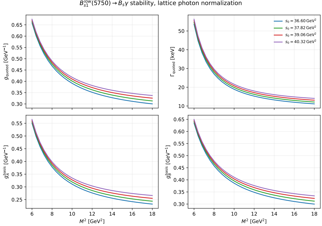
Figure 16: Redo B_{s1}^{low}(5750) \rightarrow B_s \gamma diagnostic stability curves. The lower-state prediction has a stronger monotonic M^2 dependence than the observed B_{s1}(5830) , so its quoted range should remain a model diagnostic until the corresponding state assignment and continuum window are better fixed.
