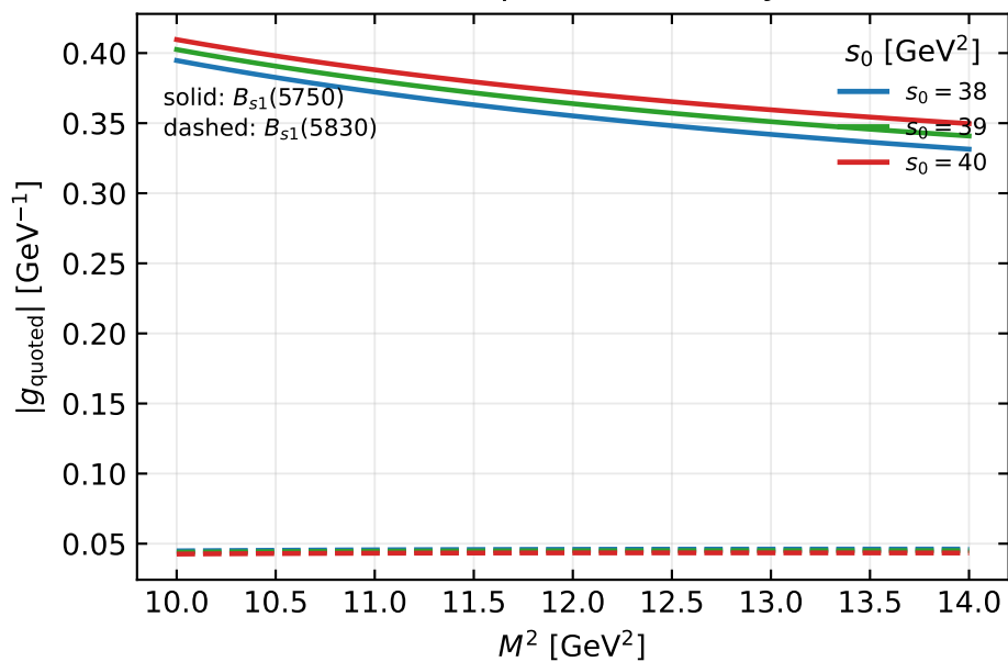
B_{s1} \rightarrow B_s \gamma : Borel stability
