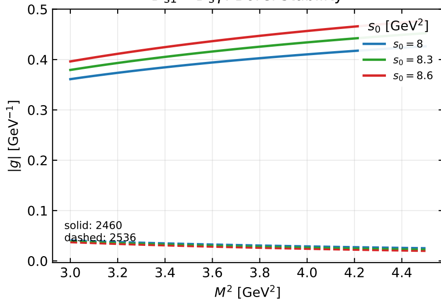
D_{s1} \rightarrow D_s \gamma : Borel stability
