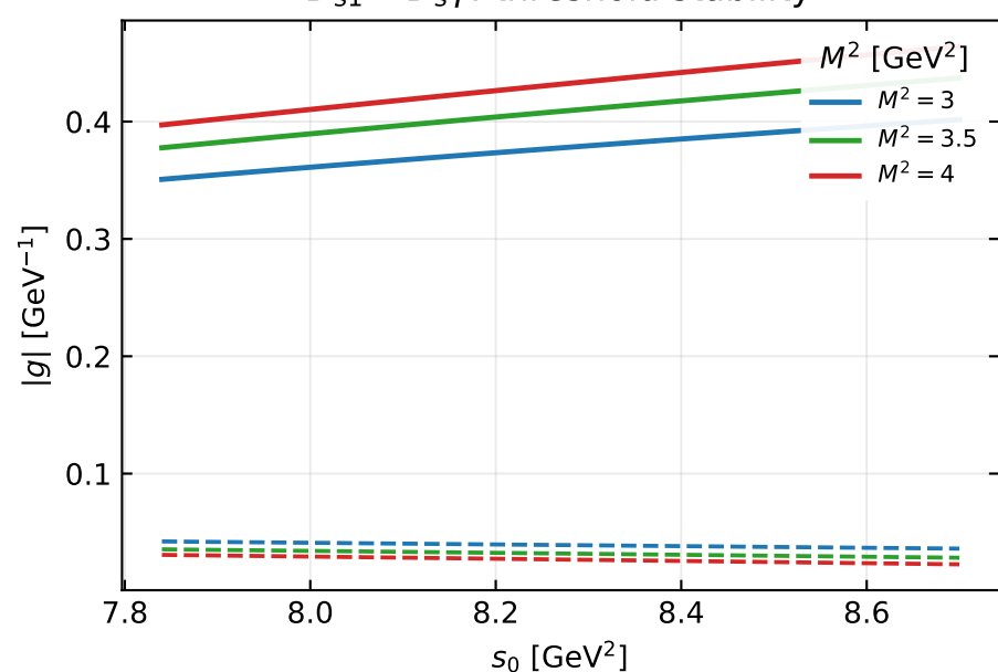
D_{s1} \rightarrow D_s \gamma : threshold stability
