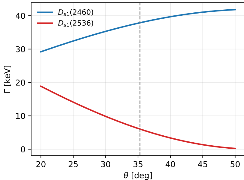
Mixing-angle dependence at M^2 = 4.5 \text{ GeV}^2 , \sqrt{s_0} = 2.55 \text{ GeV}
