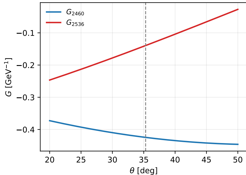
Mixing-angle dependence at M^2 = 4.5 \text{ GeV}^2 , \sqrt{s_0} = 2.55 \text{ GeV}
