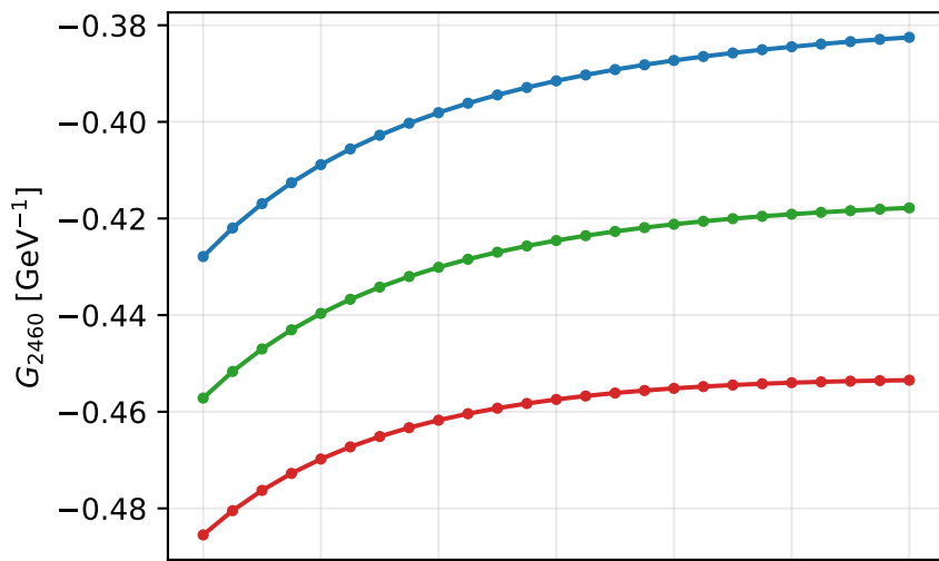
Central matched Stage-2 stability, \theta = 35.3^\circ
