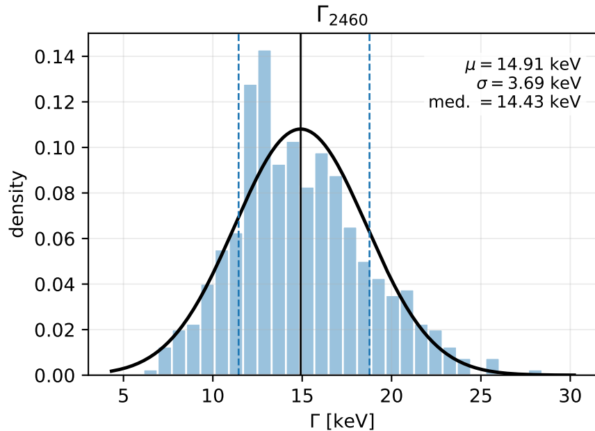
Lattice-normalized Monte Carlo width distribution, \theta = 35.3^\circ
