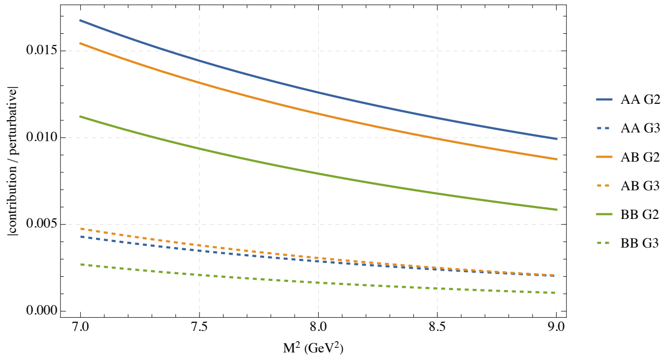
Momentum OPE hierarchy, s_0 = 53 \text{ GeV}^2
