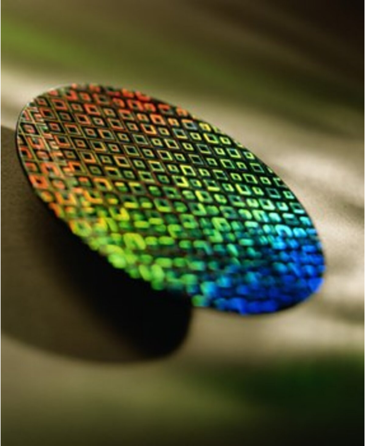
Figure C3.7: Etched Silicon Wafer Showing Individual Die
