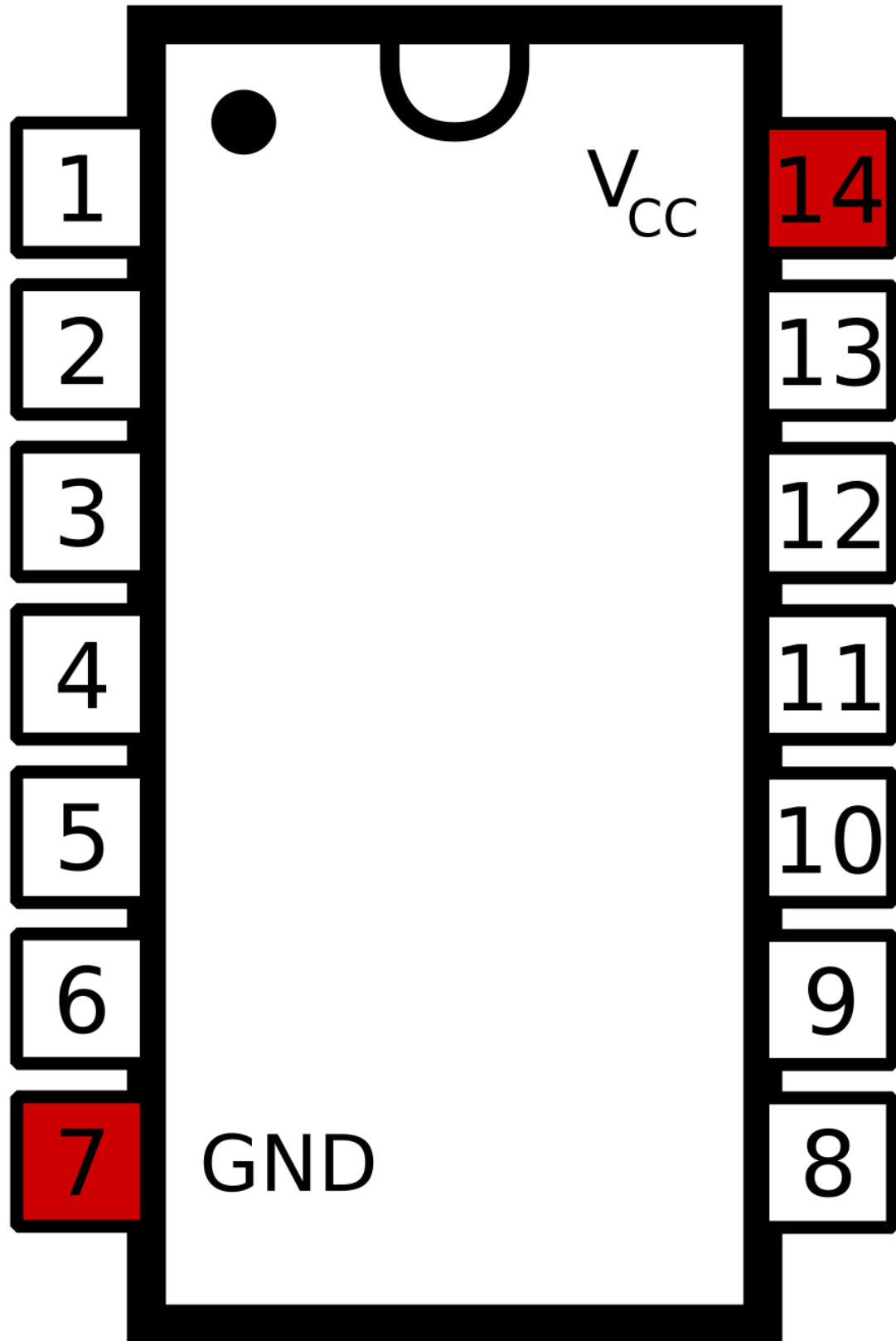
Figure C6.3 General 14-pin TTL Logic IC Pinout
