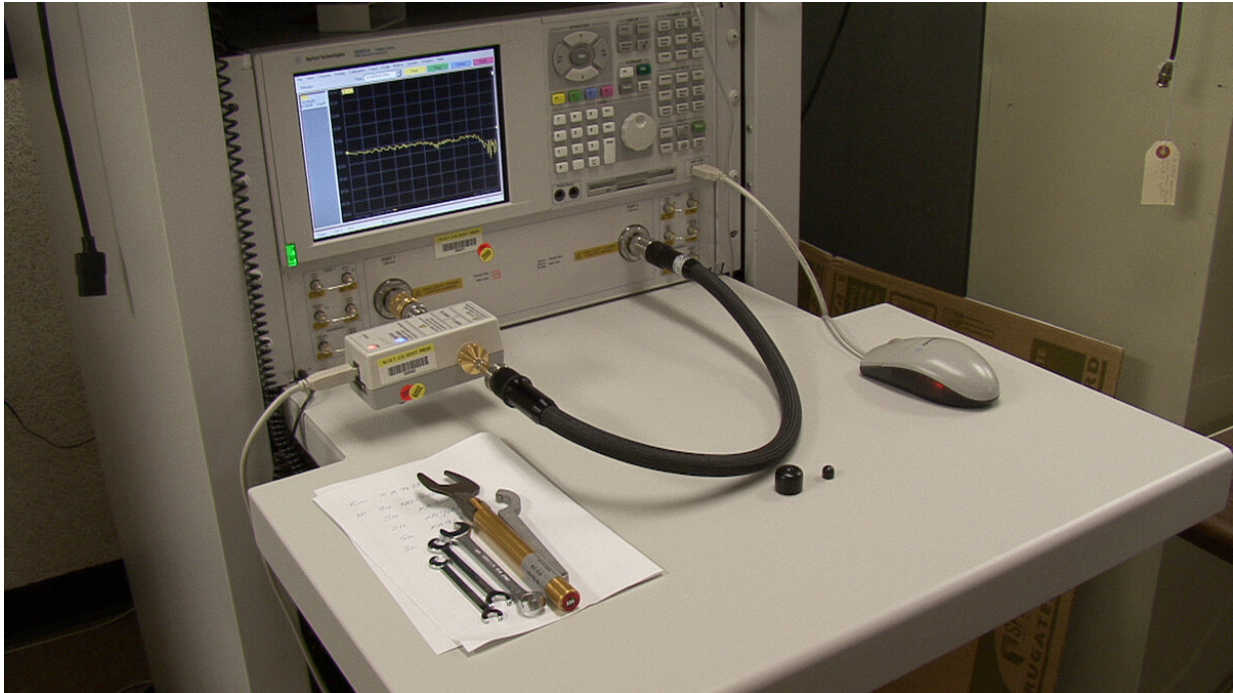
Figure C7.9: Vector Network Analyzer Used for Two-Port Network Calibration
