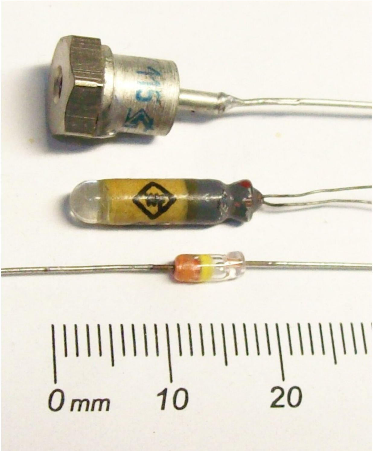
Figure C18.4: Germanium Photodiode
