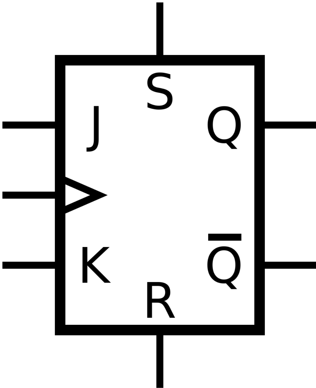
Figure C6.5: JK Flip-Flop Sequential Logic Diagram
