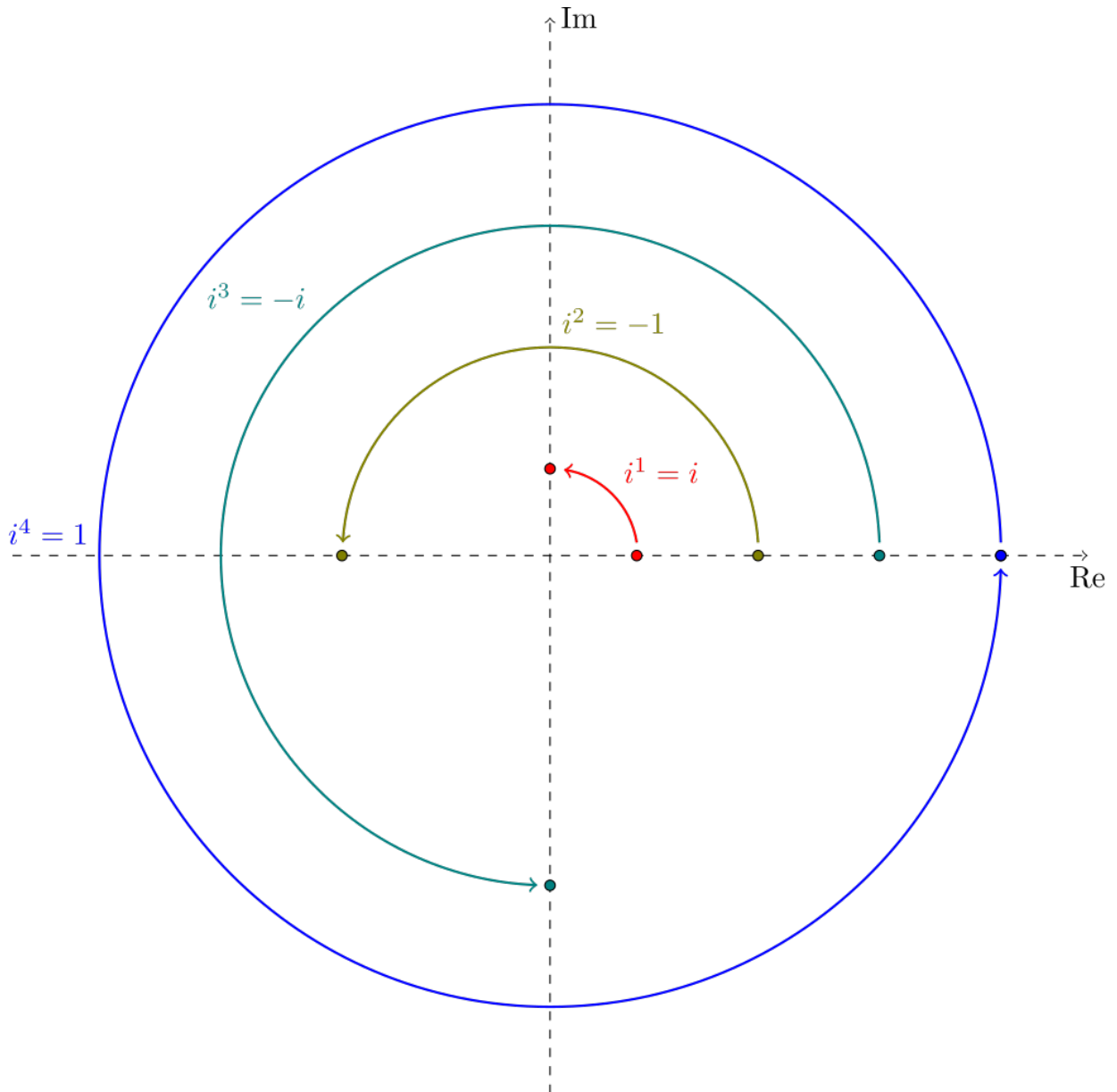
Figure C8.4: Rotations on the Complex Plane — Basis for the Z-Plane Used in the Z-Transform
