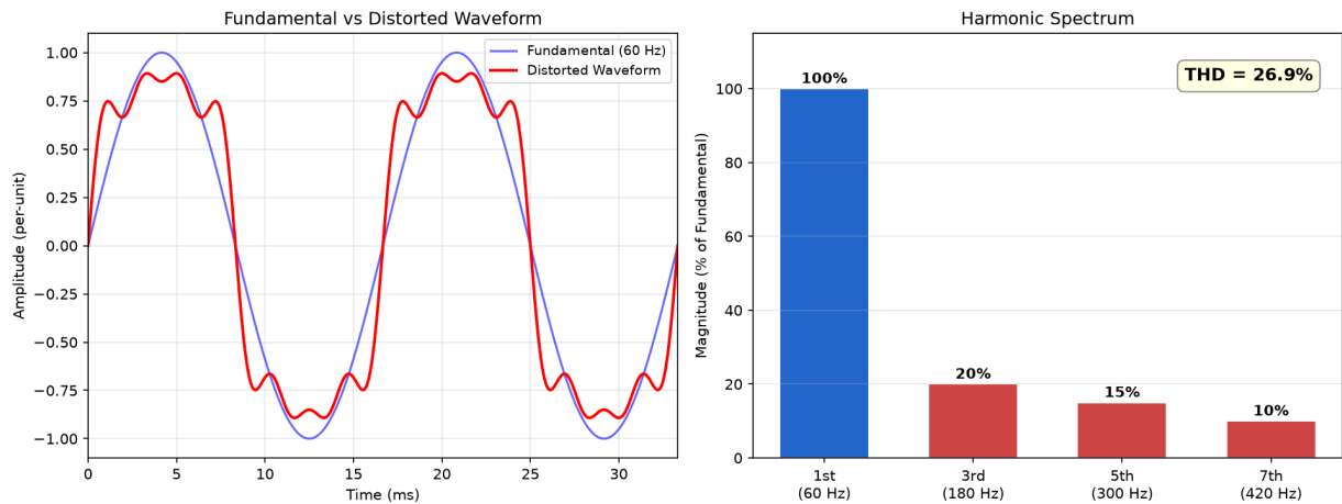
Figure 1.5.1: Harmonic Spectrum and THD
