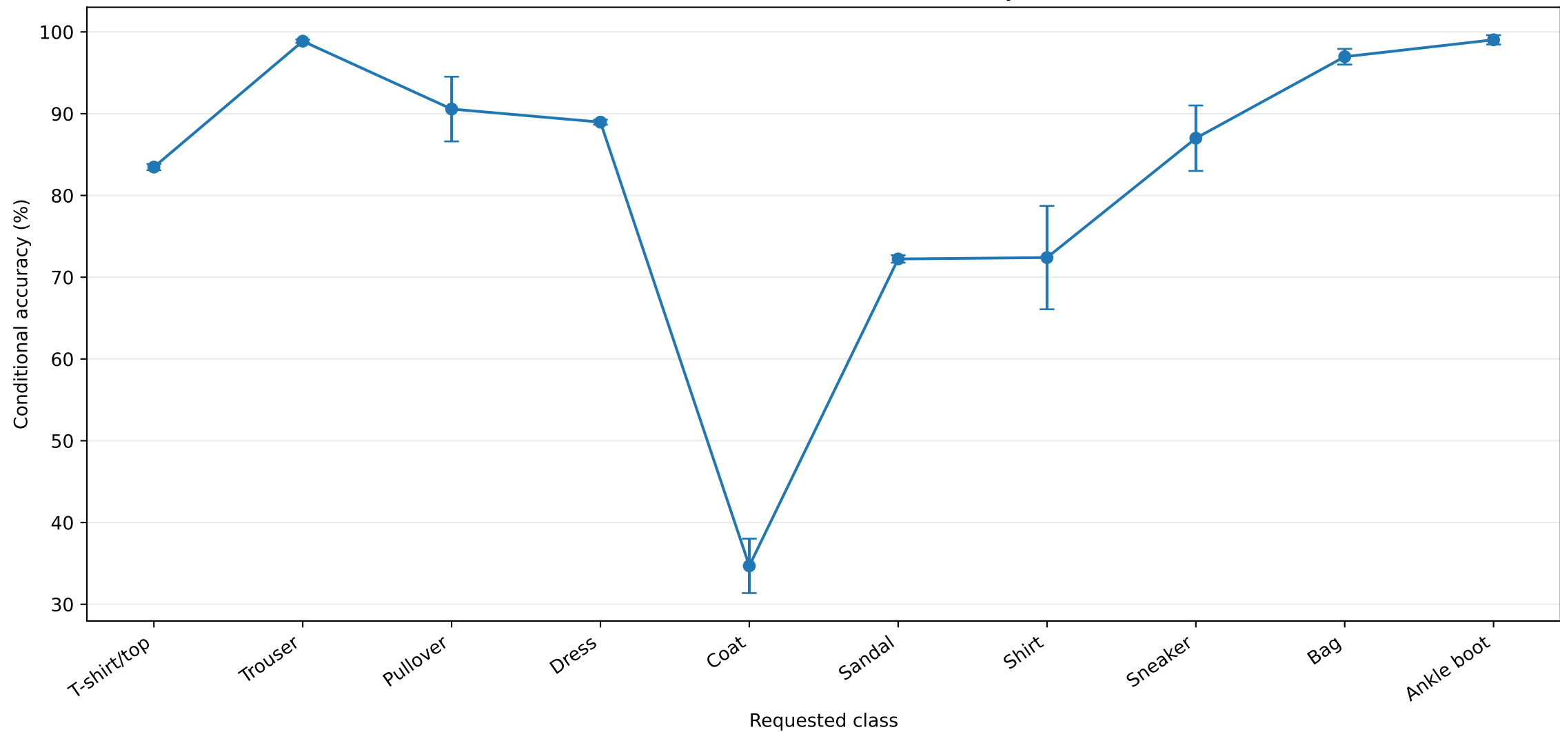
CVAE beta=1 - Conditional coherence by class
