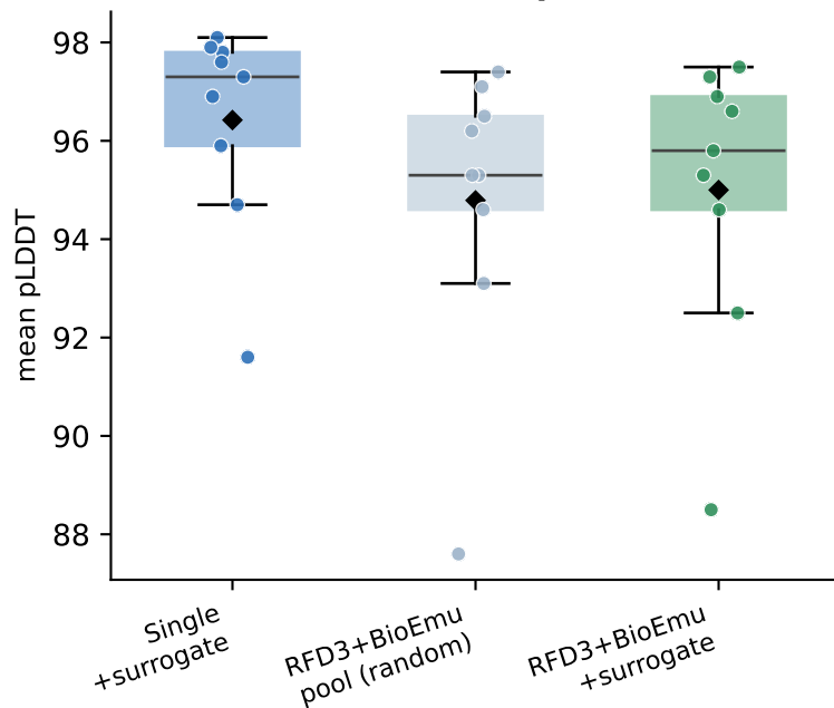
Selected-set pLDDT
