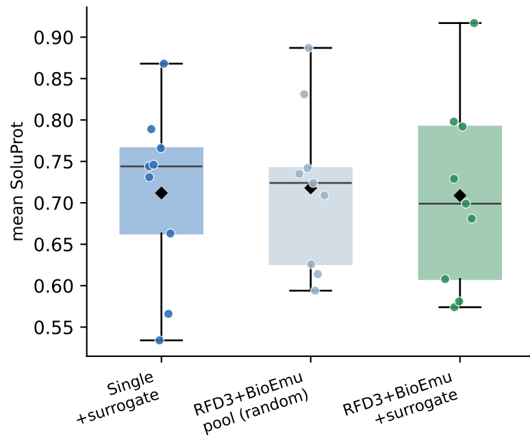
Selected-set SoluProt
