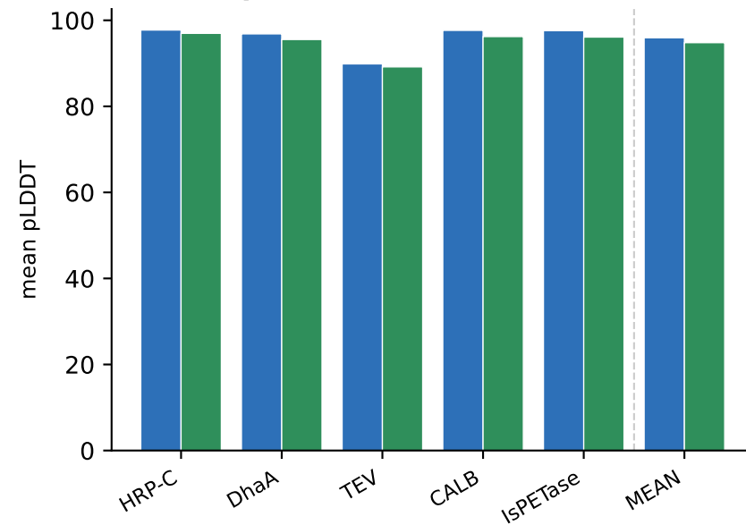
pLDDT (AF2-folded mean)
