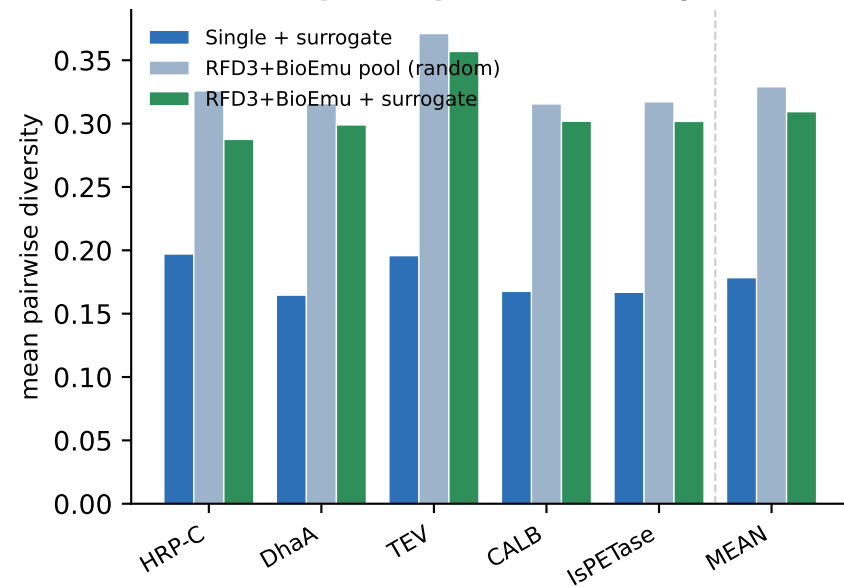
Top-K sequence diversity
