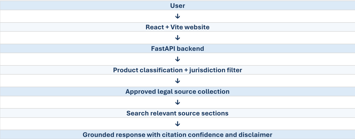
Figure 1. Target MVP architecture. The lower retrieval stages are planned, not yet implemented.
