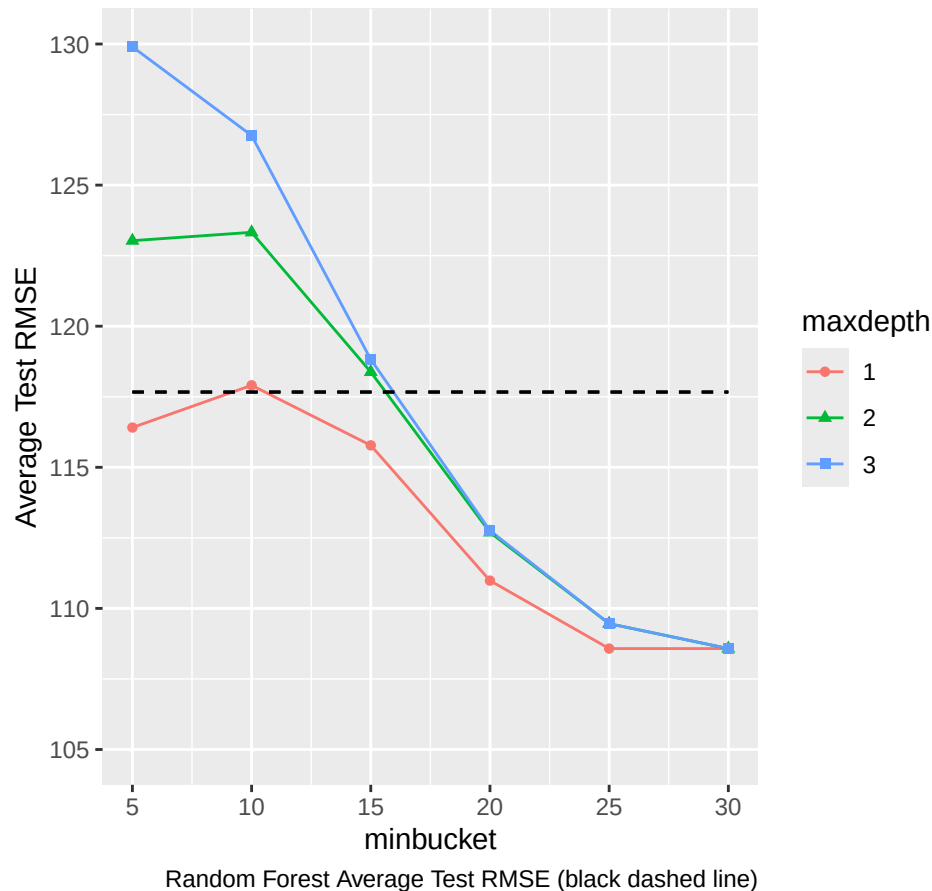
Average Test RMSE 6MWD
