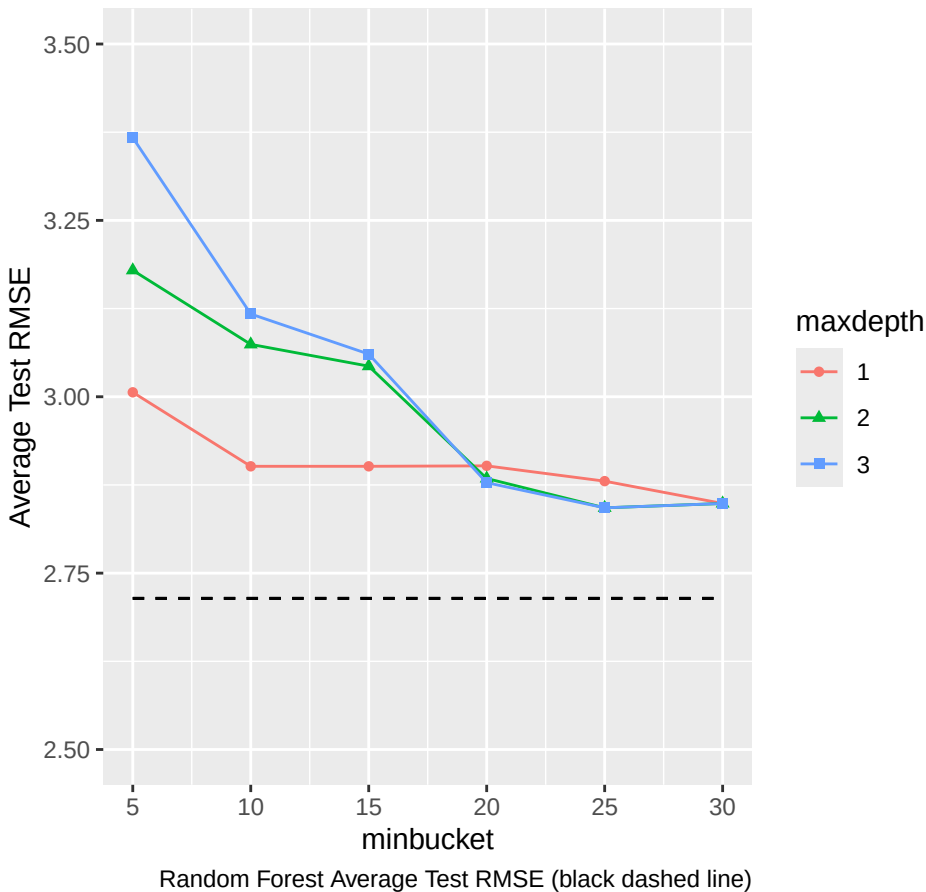
Average Test RMSE SPPB
