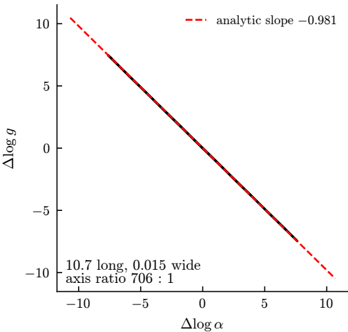
95% confidence region, true shape
