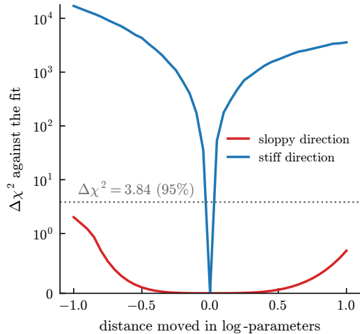
what the data notice, along each direction
