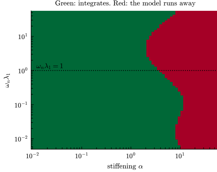
Figure 11: Where the winner can be integrated, at the fitted modulus and viscosity. Failure is governed principally by the stiffening, and the threshold falls to its lowest where the relaxation time is comparable to the bubble’s own period — but it is a boundary that moves, not an isolated band.
