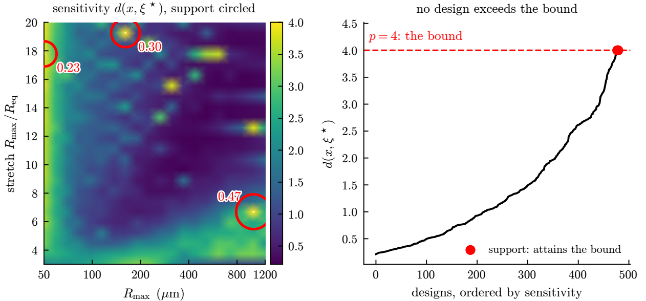
Figure 10: The equivalence-theorem certificate. Left: the sensitivity d(x, \xi^*) = \text{tr}[M(\xi^*)^{-1}M(x)] over the design plane, with the three support points circled and labelled by weight; the dashed contour is the level p = 4 . Right: the same values sorted. No design exceeds the bound and the support attains it exactly, which is the proof — \max_x d = 4.00000000 against p = 4 , gap 9 \times 10^{-10} . Nothing analogous exists for the single-design searches elsewhere in this document.
