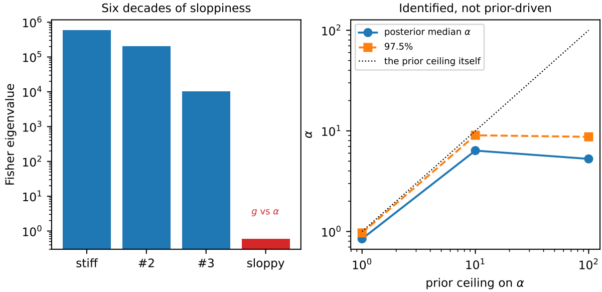
Figure 11: Left: the Fisher spectrum at the optimum, six decades between the stiffest and sloppiest directions, with the sloppiest being modulus against stiffening. Right: the posterior for \alpha against the ceiling imposed on its prior. It tracks the ceiling while truncated and departs from it once the ceiling is loose, which is what distinguishes an identified parameter from a prior-driven one.
