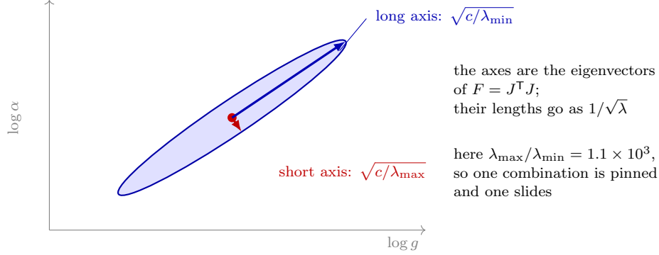
Figure 27: Why some parameter combinations are determined and others are not. Near the best fit the misfit rises as a quadratic form, so the contour of constant misfit is an ellipse whose axes point along the eigenvectors of F = J^T J and whose half-lengths go as 1/\sqrt{\lambda} . A large eigenvalue is a short axis: move that way and the fit degrades at once. A small one is a long axis: move that way and the data barely object. On these records the ratio is 1.1 \times 10^3 , and the long direction is g up with \alpha down at fixed product, which is the ridge of Figure 25 seen from above. The ellipse is drawn at an aspect of about 8 : 1; the measured aspect is \sqrt{1.1 \times 10^3} \approx 33 : 1 , which would render as a line.
