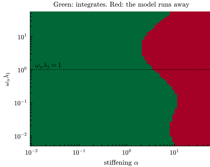
Figure 22: Where the winner can be integrated, at the fitted modulus and viscosity. Failure is governed principally by the stiffening, and the threshold falls to its lowest where the relaxation time is comparable to the bubble's own period – but it is a boundary that moves, not an isolated band.
