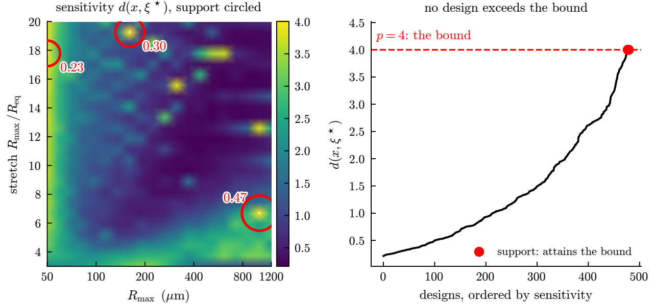
Figure 19: The equivalence-theorem certificate. Left: the sensitivity d(x, \xi^*) = \text{tr}[M(\xi^*)^{-1}M(x)] over the design plane, with the three support points circled and labeled by weight; the dashed contour is the level p = 4 . Right: the same values sorted. No design exceeds the bound and the support attains it exactly, which is the proof – \max_x d = 4.00000000 against p = 4 , gap 9 \times 10^{-10} . Nothing analogous exists for the single-design searches elsewhere in this document.
