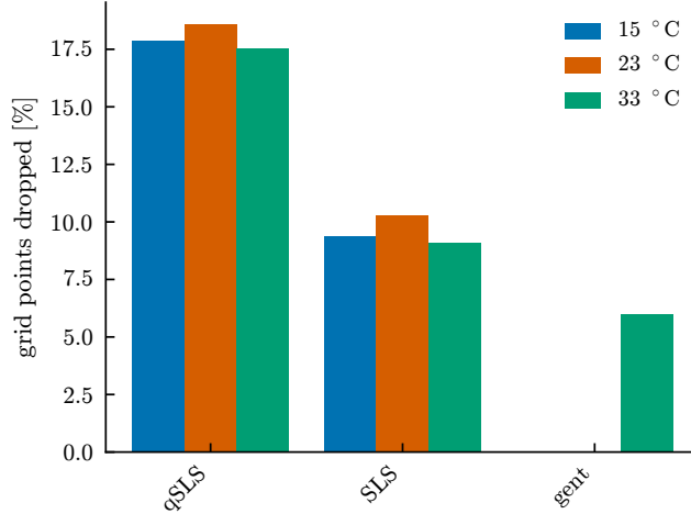
Figure 23: Fraction of each model’s parameter grid that could not be integrated. Models not shown lost no points.
