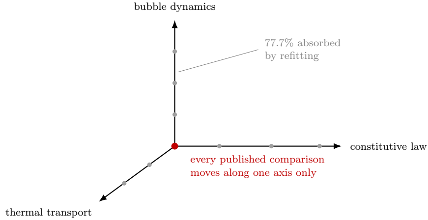
Figure 15: Three choices go into every prediction, and they are made independently: the constitutive law, the bubble-dynamics equation, and whether heat transfer is modeled. Published comparisons vary the first and leave the other two at the origin. Some of each change can be canceled by refitting stiffness and viscosity, which makes it invisible no matter how the experiment is run; what remains is 22% of an operator change, 57% of a constitutive change and 53% of a thermal one, and no two of those remainders point in similar directions. All three are therefore distinguishable in principle.
