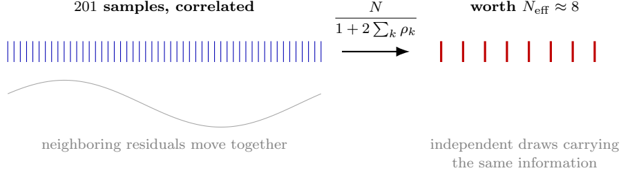
Figure 28: Why 201 samples do not carry 201 samples’ worth of evidence. The residuals here are strongly correlated from one sample to the next, so neighboring points repeat information rather than adding it. A correlated sequence carries what N_{\text{eff}} = N/(1 + 2 \sum_k \rho_k) independent draws would, and on these fits N_{\text{eff}} is near 8. Both \chi^2/N and the evidence assume the samples are independent, so each overstates the information by roughly N/N_{\text{eff}} \approx 25 . A margin of a few nats between two models is inside that factor.
