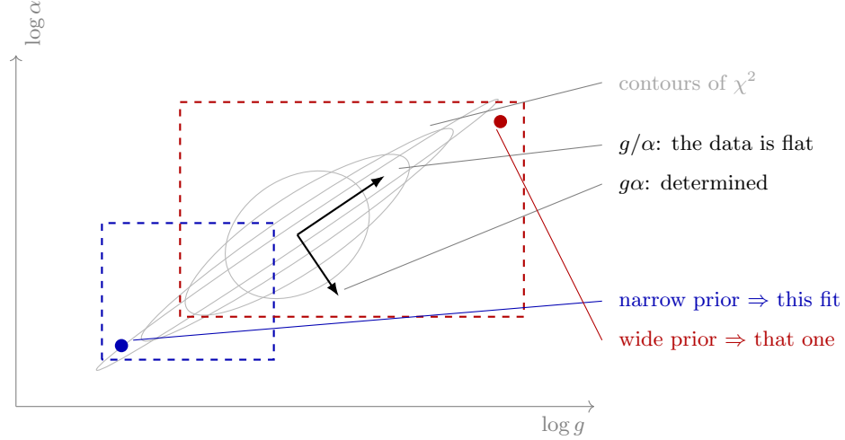
Figure 17: Why a “best fit” for g is a statement about the prior. The likelihood depends on the product g\alpha , so the misfit surface is a valley running along constant g\alpha and the data is flat along g/\alpha . An optimiser slides until it meets the edge of the box, and where it stops is set by the box: the two dashed rectangles give the two filled points, which differ in g by more than thirtyfold. This is the mechanism behind the fifty-nat swing in the operator ranking of §4 when the bounds were widened, and behind the order-of-magnitude disagreement in g between methods in Fig. 9.
