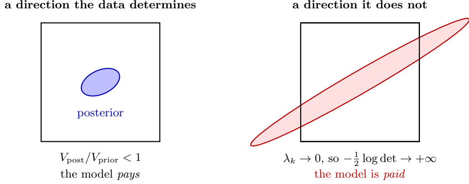
Figure 16: The Occam factor is the share of the prior the data leaves standing, \prod_k \sqrt{2\pi/\lambda_k} over the eigenvalues of J^\top J . Left: every direction is narrower than its prior, so a flexible model pays for volume it does not use. Right: a direction the data does not determine has \lambda_k \rightarrow 0 , the fitted Gaussian extends far outside the box the prior occupies, and the expansion returns a factor greater than one — the evidence rises when a useless parameter is added. Capping each direction at unity, (45), restores what the geometry already required; on the models of §3.4 the uncapped form favoured the two-mode law by 29.7 nats exactly where its second arm did nothing.
