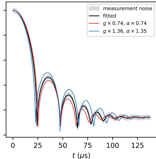
The same change in the parameters, seen by the data two ways along the SLOPPY direction
