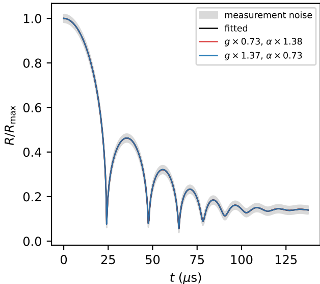
The same change in the parameters, seen by the data two ways along the SLOPPY direction
