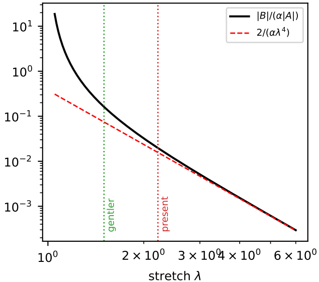
Separability dies as \lambda^{-4}
