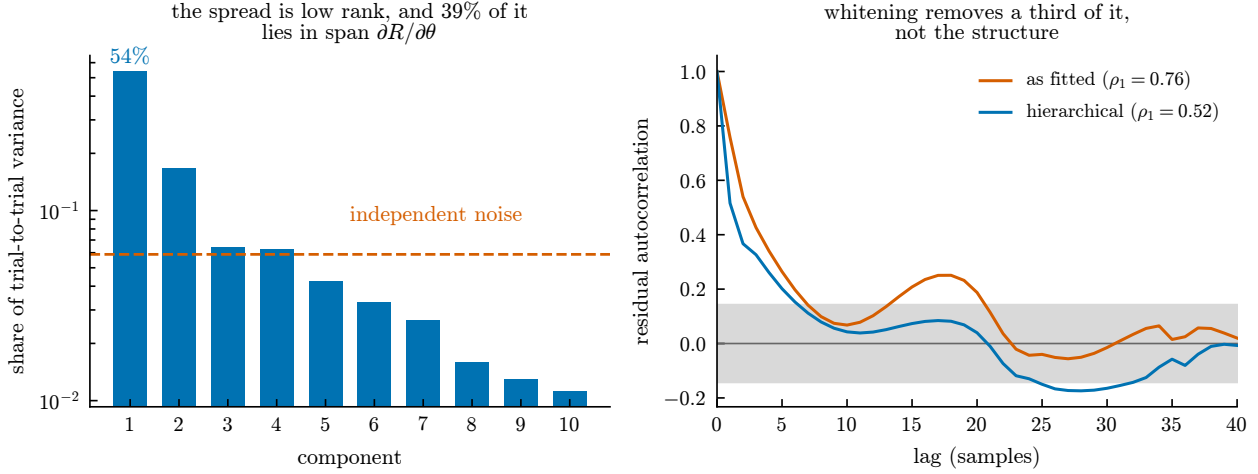
Figure 4: What the trial spread is, and what it does not explain. Left: the singular spectrum of the eighteen trial deviations. Independent measurement error would put an equal share in every component (dashed); instead the leading one carries 54%, and 39% of the total lies in the six-dimensional span of \partial R/\partial \theta against a 3% chance level. Right: the autocorrelation of the qSLS fit residual before and after whitening by the hierarchical covariance (11), with the white-noise band shaded. If the correlation were caused by variation between bubbles, whitening would flatten it into that band. It removes about a third and leaves the rest, so the remainder is structure the model does not contain.
