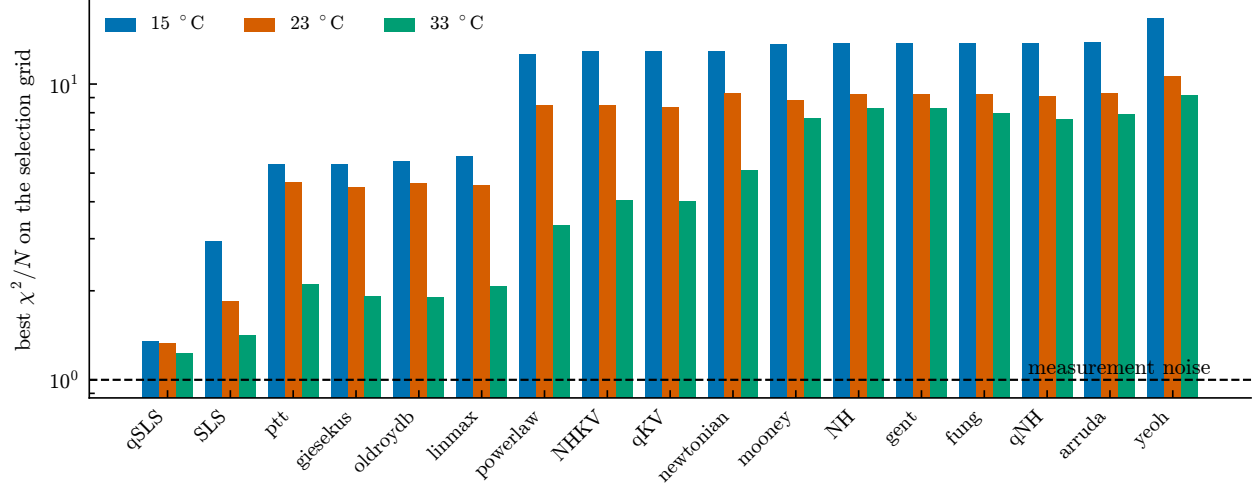
Figure 2: Best \chi^2/N on the selection grid for every candidate, all three temperatures, logarithmic scale. The dashed line is the measurement-noise floor.
