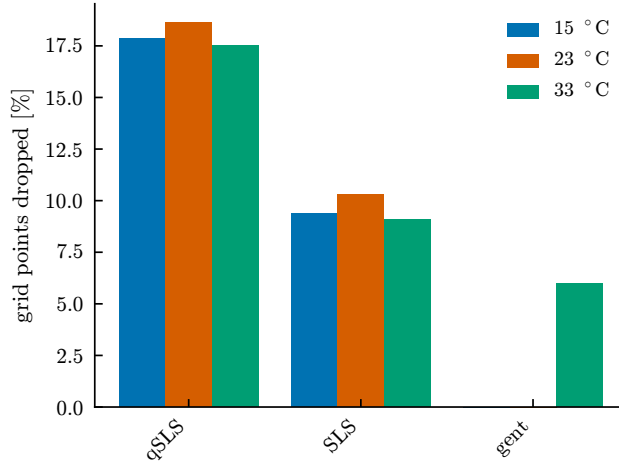
Figure 15: Fraction of each model’s parameter grid that could not be integrated. Models not shown lost no points.
