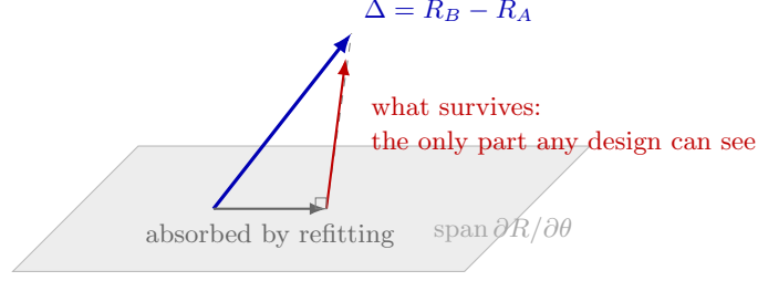
Figure 13: Why a model difference can be invisible at every design. Changing a model perturbs the trace by \Delta = R_B - R_A . The component of \Delta lying in the span of the material sensitivities is reproduced by adjusting g, \mu, \lambda_1, \alpha — refitting absorbs it, and no experiment recovers it. Only the orthogonal remainder is evidence that the model changed. Measured on the 15 °C record and reported in §5: the bubble-dynamics operator is 77.7% absorbed, leaving under two noise units, which is why its ranking proved so fragile; the constitutive and thermal axes leave 8.1 and 8.5.
