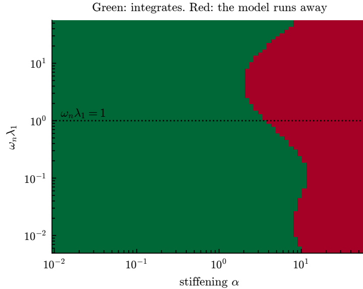
Figure 14: Where the winner can be integrated, at the fitted modulus and viscosity. Failure is governed principally by the stiffening, and the threshold falls to its lowest where the relaxation time is comparable to the bubble’s own period — but it is a boundary that moves, not an isolated band.
