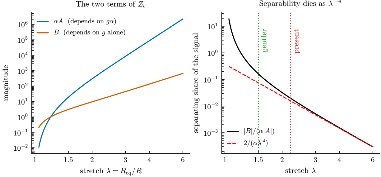
Figure 6: The two terms of (15) against collapse depth. Left: \alpha A , which depends on the product g\alpha , outruns B , which carries g alone. Right: their ratio, the share of the signal that can separate the two parameters, following 2/(\alpha\lambda^4) once the collapse is deep. It is 2% at the depth these records reach and 16% at \lambda = 1.5 .
