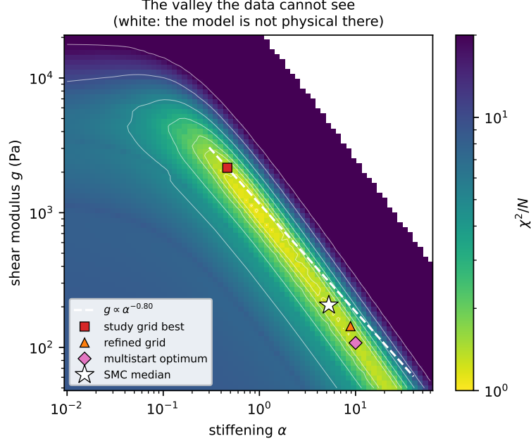
Figure 7: \chi^2/N over the modulus–stiffening plane, at the fitted viscosity and relaxation time. The dashed line is g \propto \alpha^{-0.80} , predicted from the Fisher curvature at a single point; it lies along the floor of the valley. Four “best fits” from four methods are strung out along that floor rather than disagreeing with one another. The white region at upper right is where the model is not physical.
