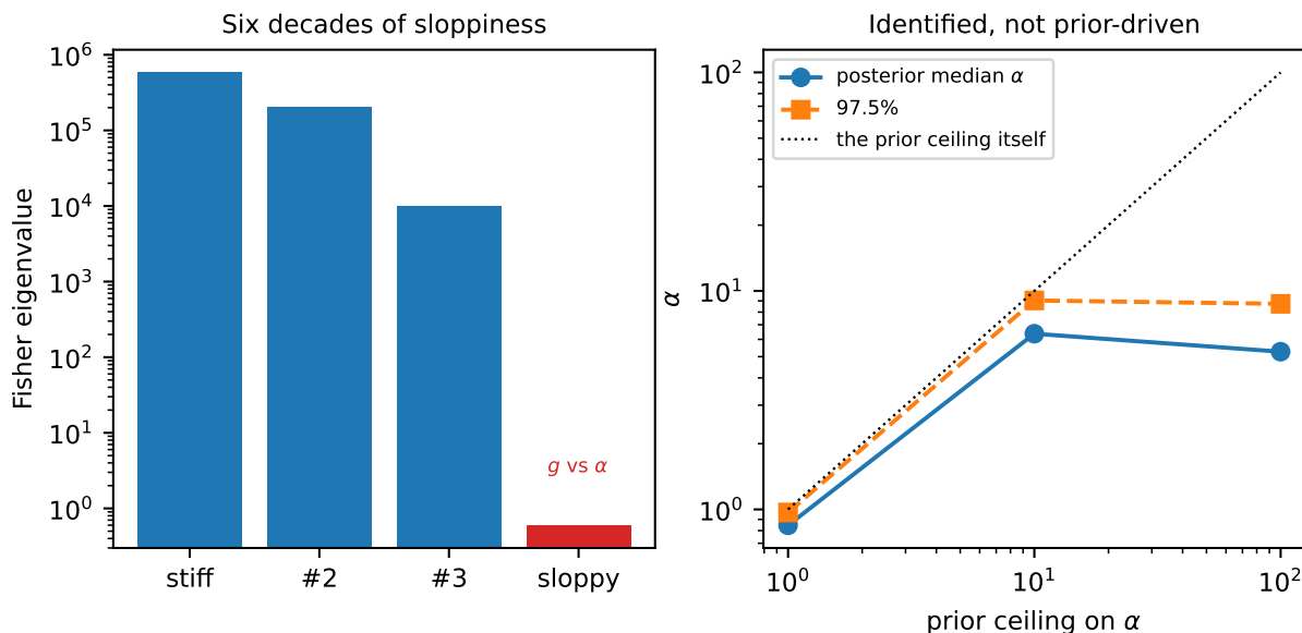
Figure 8: Left: the Fisher spectrum at the optimum, six decades between the stiffest and sloppiest directions, with the sloppiest being modulus against stiffening. Right: the posterior for \alpha against the ceiling imposed on its prior. It tracks the ceiling while truncated and departs from it once the ceiling is loose, which is what distinguishes an identified parameter from a prior-driven one.
