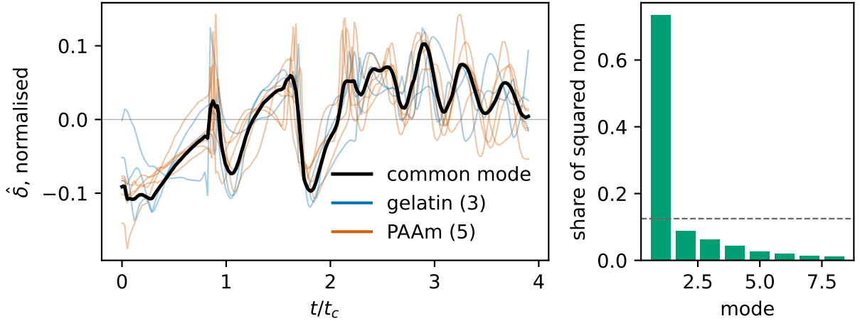
Figure 12: The discrepancy every model in this document leaves behind. Left: the eight \hat{\delta} , normalised and signed onto their common mode, gelatin in blue and PAAm in orange, with the mode in black. Right: the singular spectrum, against the 1/8 an unrelated set would give (dashed). The mode is tabulated in universal_curve.json so it can be read off rather than re-derived.
