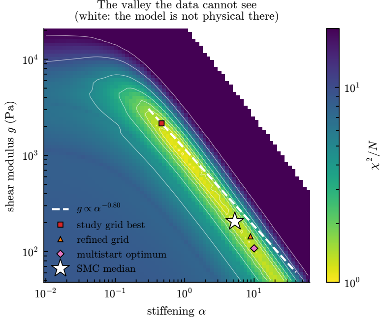
Figure 12: \chi^2/N over the modulus–stiffening plane, at the fitted viscosity and relaxation time. The dashed line is g \propto \alpha^{-0.80} , predicted from the Fisher curvature at a single point; it lies along the floor of the valley. Four “best fits” from four methods are strung out along that floor rather than disagreeing with one another. The white region at upper right is where the model is not physical.
