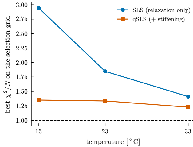
Figure 20: What the stiffening term buys, against temperature. The advantage of qSLS over SLS narrows as the gel warms.
