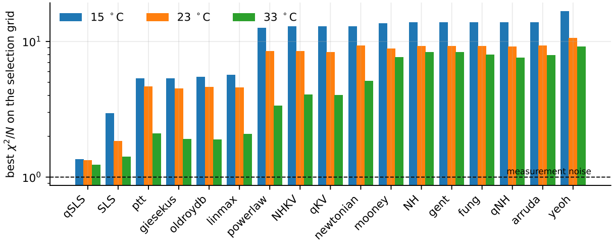
Figure 2: Best \chi^2/N on the selection grid for every candidate, all three temperatures, logarithmic scale. The dashed line is the measurement-noise floor.
