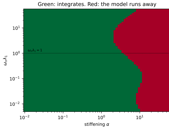
Figure 11: Where the winner can be integrated, at the fitted modulus and viscosity. Failure is governed principally by the stiffening, and the threshold falls to its lowest where the relaxation time is comparable to the bubble’s own period — but it is a boundary that moves, not an isolated band.
