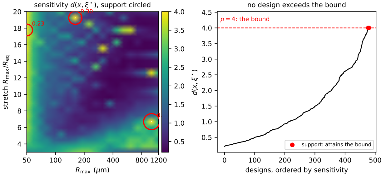
Figure 10: The equivalence-theorem certificate. Left: the sensitivity d(x, \xi^*) = \text{tr}[M(\xi^*)^{-1}M(x)] over the design plane, with the three support points circled and labelled by weight; the dashed contour is the level p = 4 . Right: the same values sorted. No design exceeds the bound and the support attains it exactly, which is the proof — \max_x d = 4.00000000 against p = 4 , gap 9 \times 10^{-10} . Nothing analogous exists for the single-design searches elsewhere in this document.
