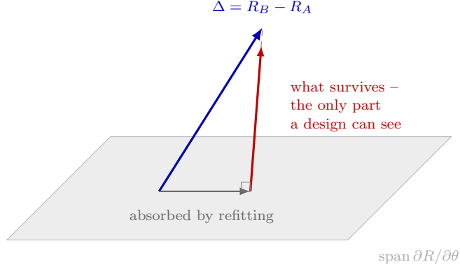
Figure 17: Why a model difference can be invisible at every design. Changing a model perturbs the trace by \Delta = R_B - R_A . The component lying in the span of the material sensitivities is reproduced by adjusting g, \mu, \lambda_1, \alpha – refitting absorbs it, and no experiment recovers it. Only the orthogonal remainder is evidence that the model changed. Measured on the 15 °C record and reported in Section 7: the bubble-dynamics operator is 77.7% absorbed, leaving under two noise units, which is why its ranking proved so fragile; the constitutive and thermal axes leave 8.1 and 8.5.
