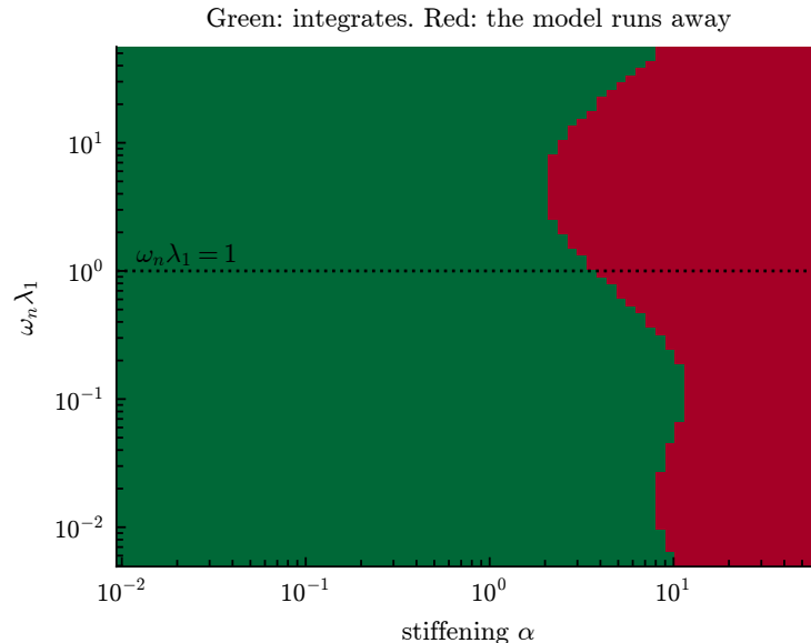
Figure 19: Where the winner can be integrated, at the fitted modulus and viscosity. Failure is governed principally by the stiffening, and the threshold falls to its lowest where the relaxation time is comparable to the bubble’s own period – but it is a boundary that moves, not an isolated band.
