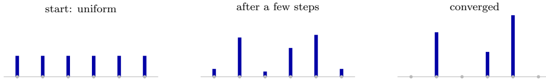
Figure 24: How the optimal design is found. Every candidate starts with equal weight, and each step multiplies a candidate's weight by how informative it is relative to the current average, then renormalizes. Weights therefore stay positive and keep summing to one by construction, and the criterion increases at every step. Candidates that are not worth running decay to zero, so the answer is a handful of settings out of hundreds. The final weights are the fraction of bubbles to run at each setting, and Figure 22 is what certifies that no other allocation does better.
