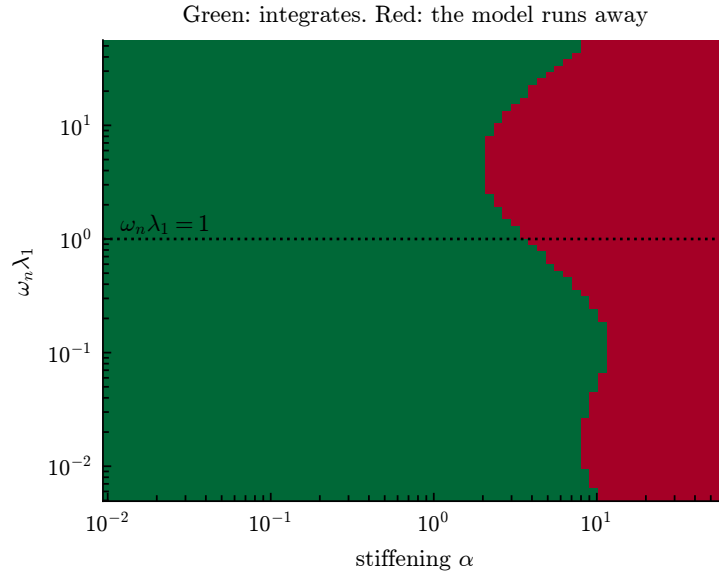
Figure 12: Where the winner can be integrated, at the fitted modulus and viscosity. Failure is governed principally by the stiffening, and the threshold falls to its lowest where the relaxation time is comparable to the bubble’s own period — but it is a boundary that moves, not an isolated band.
