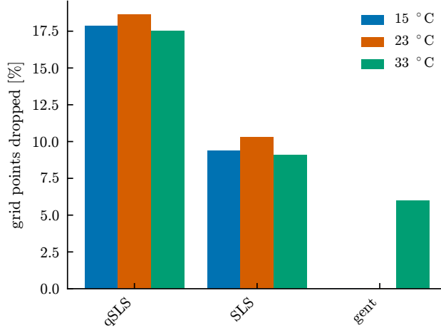
Figure 13: Fraction of each model’s parameter grid that could not be integrated. Models not shown lost no points.
