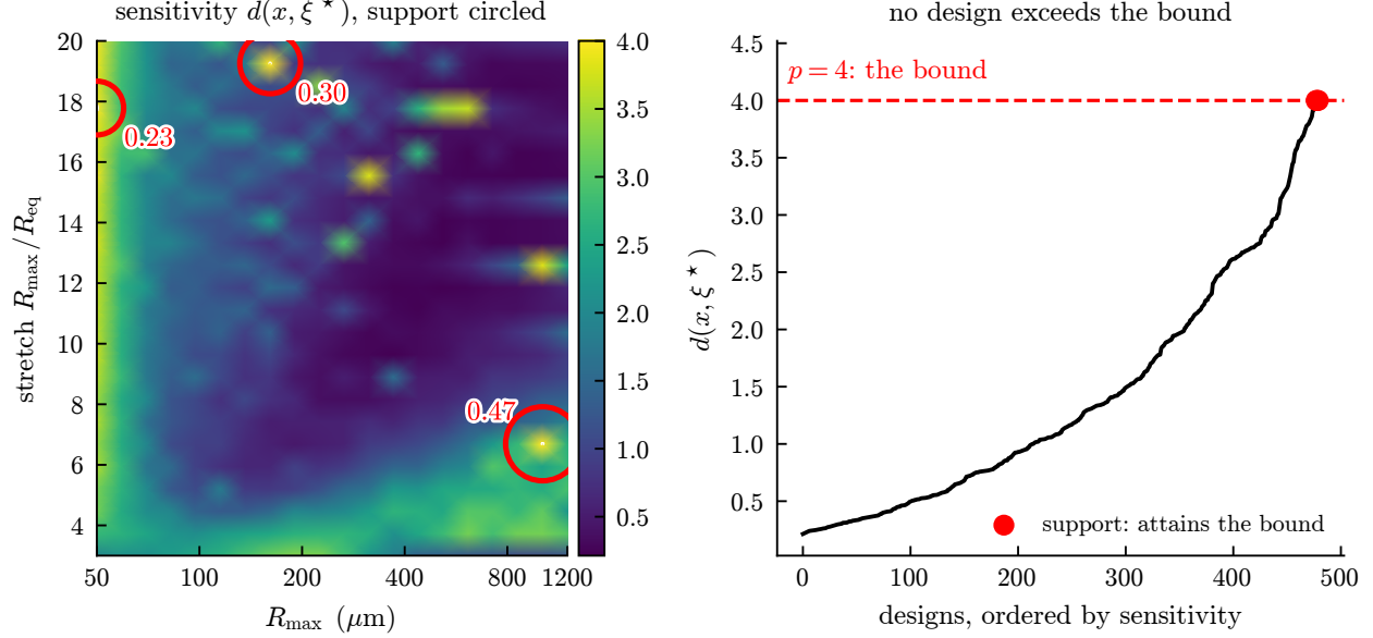
Figure 15: The equivalence-theorem certificate. Left: the sensitivity d(x, \xi^*) = \text{tr}[M(\xi^*)^{-1}M(x)] over the design plane, with the three support points circled and labelled by weight; the dashed contour is the level p = 4 . Right: the same values sorted. No design exceeds the bound and the support attains it exactly, which is the proof — \max_x d = 4.00000000 against p = 4 , gap 9 \times 10^{-10} . Nothing analogous exists for the single-design searches elsewhere in this document.
