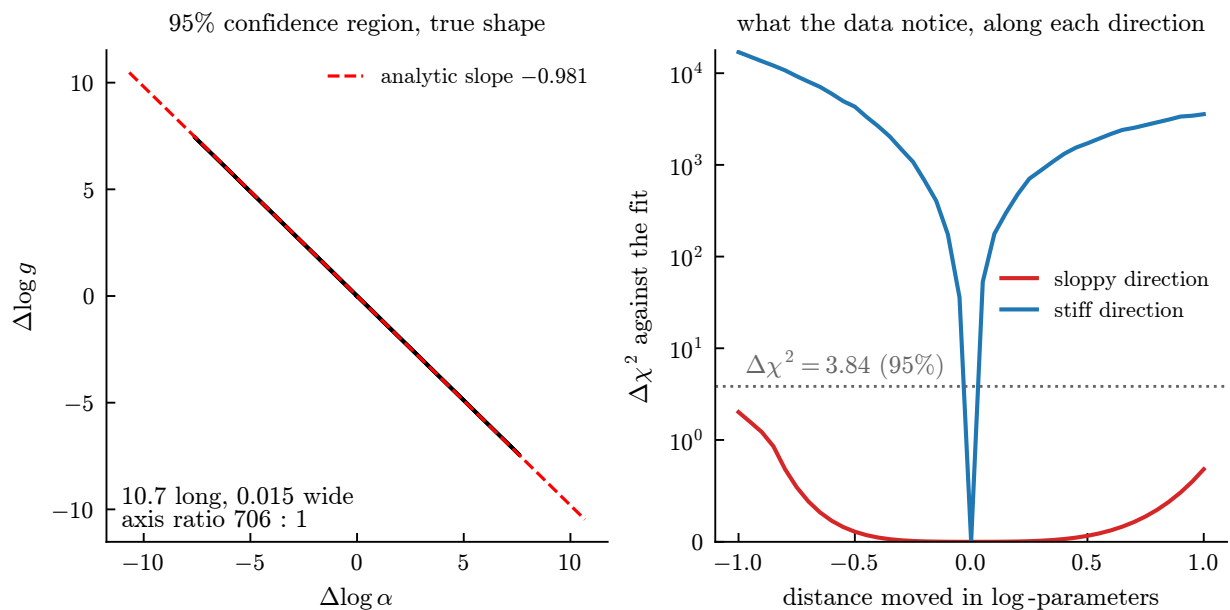
Figure 11: Left: the 95% region from the inverse Fisher information, 10.7 long and 0.015 wide in log-parameters — an axis ratio of 706, which is why it draws as a line, and the analytic slope of -0.981 lies along it. Right: the misfit measured by re-solving at perturbed parameters, not the quadratic approximation. Moving along the stiff direction costs 10^4 in \Delta\chi^2 ; moving the same distance along the sloppy one stays below the 95% threshold, so the parameters may shift by a factor of e \approx 2.7 without the data objecting.
