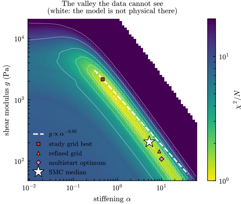
Figure 12: \chi^2/N over the modulus–stiffening plane, at the fitted viscosity and relaxation time. The dashed line is g \propto \alpha^{-0.80} , predicted from the Fisher curvature at a single point; it lies along the floor of the valley. Four “best fits” from four methods are strung out along that floor rather than disagreeing with one another. The white region at upper right is where the model is not physical.
