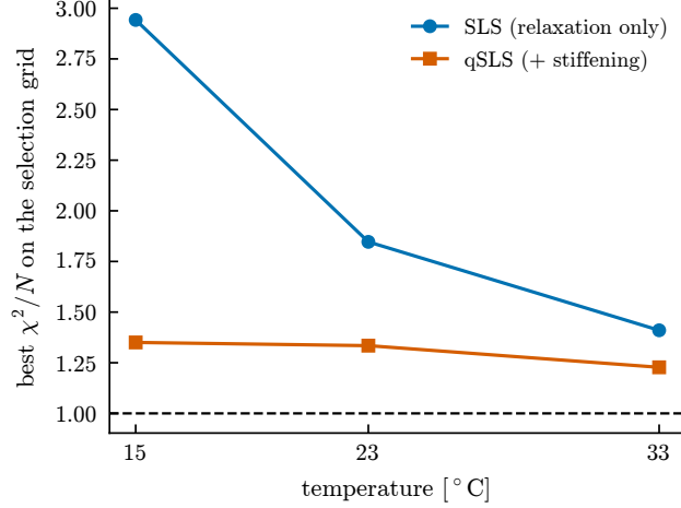
Figure 8: What the stiffening term buys, against temperature. The advantage of qSLS over SLS narrows as the gel warms.
