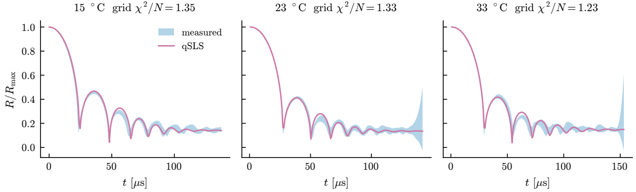
Figure 6: The selected model against the measured band it was fitted to.
