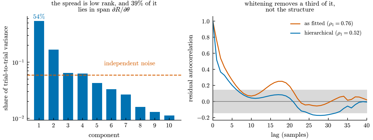
Figure 7: What the trial spread is, and what it does not explain. Left: the singular spectrum of the eighteen trial deviations. Independent measurement error would put an equal share in every component (dashed); instead the leading one carries 54%, and 39% of the total lies in the six-dimensional span of \partial R/\partial \theta against a 3% chance level. Right: the autocorrelation of the qSLS fit residual before and after whitening by the hierarchical covariance (11), with the white-noise band shaded. If the correlation were caused by variation between bubbles, whitening would flatten it into that band. It removes about a third and leaves the rest, so the remainder is structure the model does not contain.
