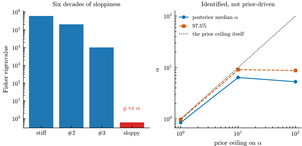
Figure 13: Left: the Fisher spectrum at the optimum, six decades between the stiffest and sloppiest directions, with the sloppiest being modulus against stiffening. Right: the posterior for \alpha against the ceiling imposed on its prior. It tracks the ceiling while truncated and departs from it once the ceiling is loose, which is what distinguishes an identified parameter from a prior-driven one.
