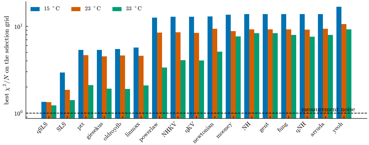
Figure 5: Best \chi^2/N on the selection grid for every candidate, all three temperatures, logarithmic scale. The dashed line is the measurement-noise floor.
