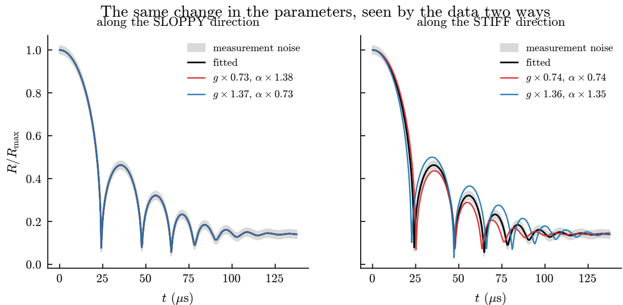
Figure 10: What an eigenvector means, shown rather than defined. The parameters are moved the same distance in log-space along each eigenvector. Along the sloppy direction a 27% change in the modulus, compensated by 38% in the stiffening, leaves the trajectory inside the measurement noise; along the stiff direction a change of the same size is obvious. The data cannot see the first and cannot miss the second.
