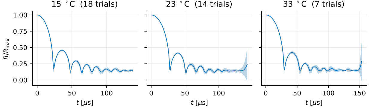
Figure 1: Measured records. Line is the mean over trials, band is \pm one standard deviation across trials at each time. The spread is the noise model.
