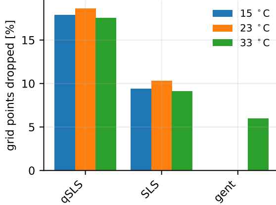
Figure 11: Fraction of each model’s parameter grid that could not be integrated. Models not shown lost no points.
