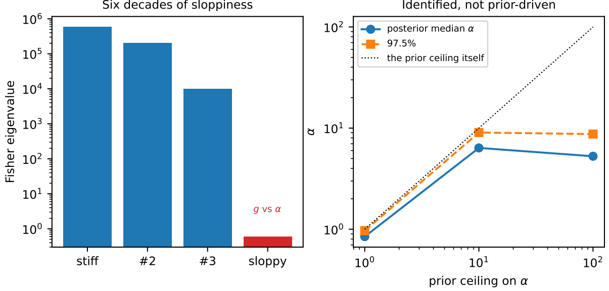
Figure 9: Left: the Fisher spectrum at the optimum, six decades between the stiffest and sloppiest directions, with the sloppiest being modulus against stiffening. Right: the posterior for \alpha against the ceiling imposed on its prior. It tracks the ceiling while truncated and departs from it once the ceiling is loose, which is what distinguishes an identified parameter from a prior-driven one.
