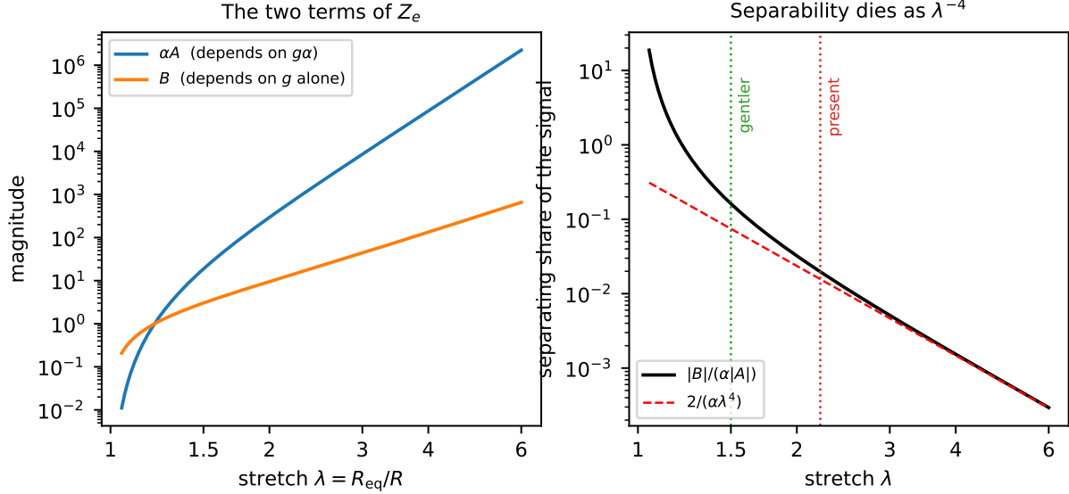
Figure 5: The two terms of (13) against collapse depth. Left: \alpha A , which depends on the product g\alpha , outruns B , which carries g alone. Right: their ratio, the share of the signal that can separate the two parameters, following 2/(\alpha\lambda^4) once the collapse is deep. It is 2% at the depth these records reach and 16% at \lambda = 1.5 .
