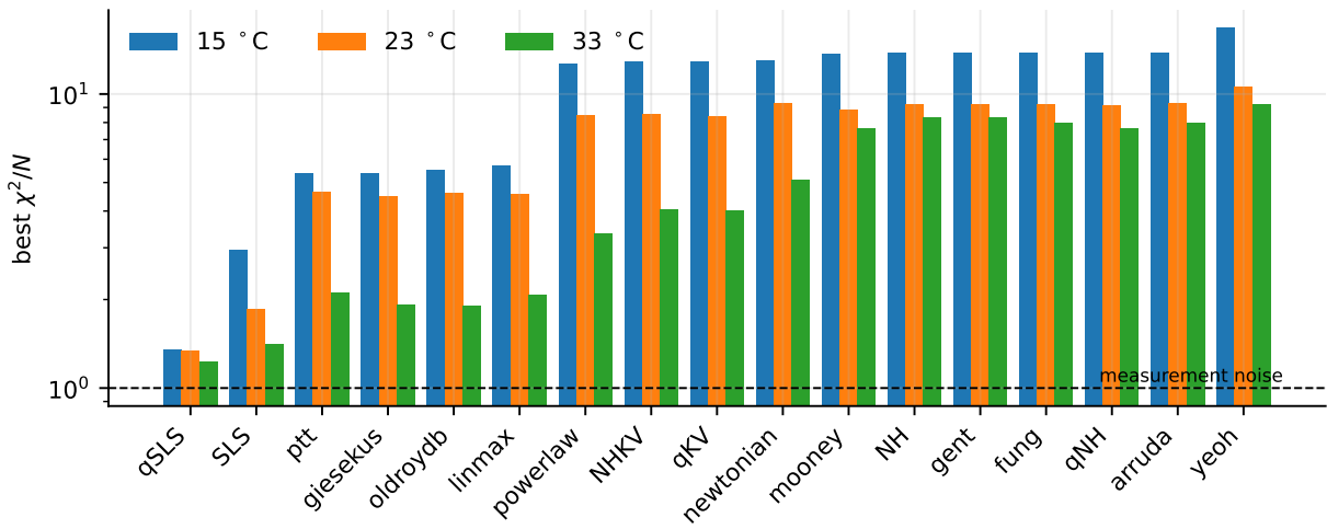
Figure 2: Best \chi^2/N for every candidate, all three temperatures, logarithmic scale. The dashed line is the measurement-noise floor.
