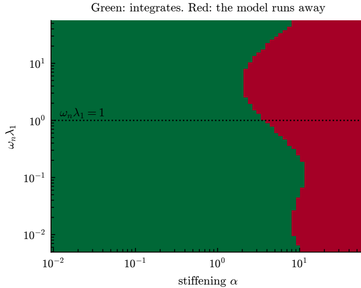
Figure 20: Where the winner can be integrated, at the fitted modulus and viscosity. Failure is governed principally by the stiffening, and the threshold falls to its lowest where the relaxation time is comparable to the bubble’s own period – but it is a boundary that moves, not an isolated band.
