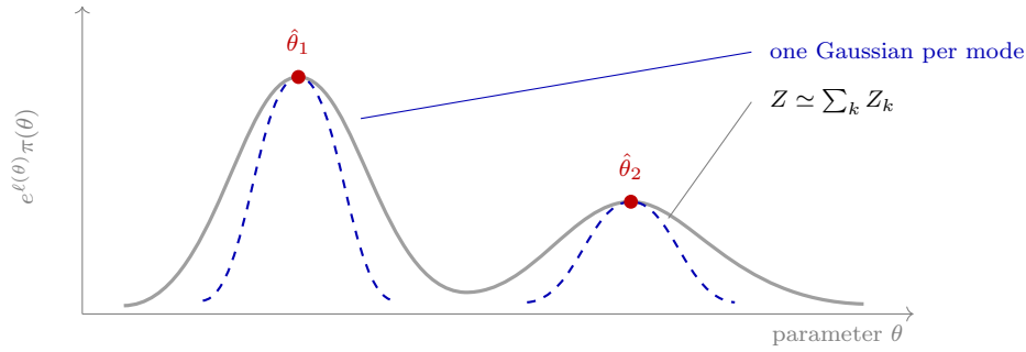
Figure 3: The Laplace expansion, and why the evidence is summed over modes. The integrand e^{\ell}\pi is expanded about each maximum as a Gaussian, whose height and width give that mode’s contribution Z_k in closed form; the evidence is \sum_k Z_k , computed as a logsumexp over the distinct endpoints a multistart finds. Taking only the best mode discards the rest of the integral, which is the difference between an integral criterion and a minimum: a missed mode biases the total slightly, where a missed basin corrupts a minimum entirely. This is why fit_candidate returns every distinct endpoint rather than its winner.
