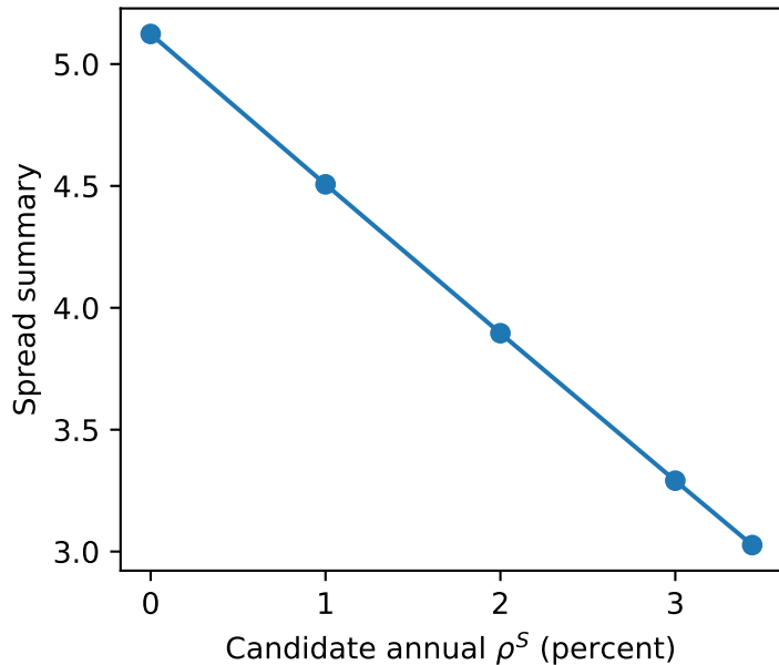
Fiberwise log-spread
