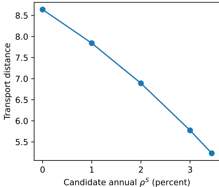
Conditional transport distance
