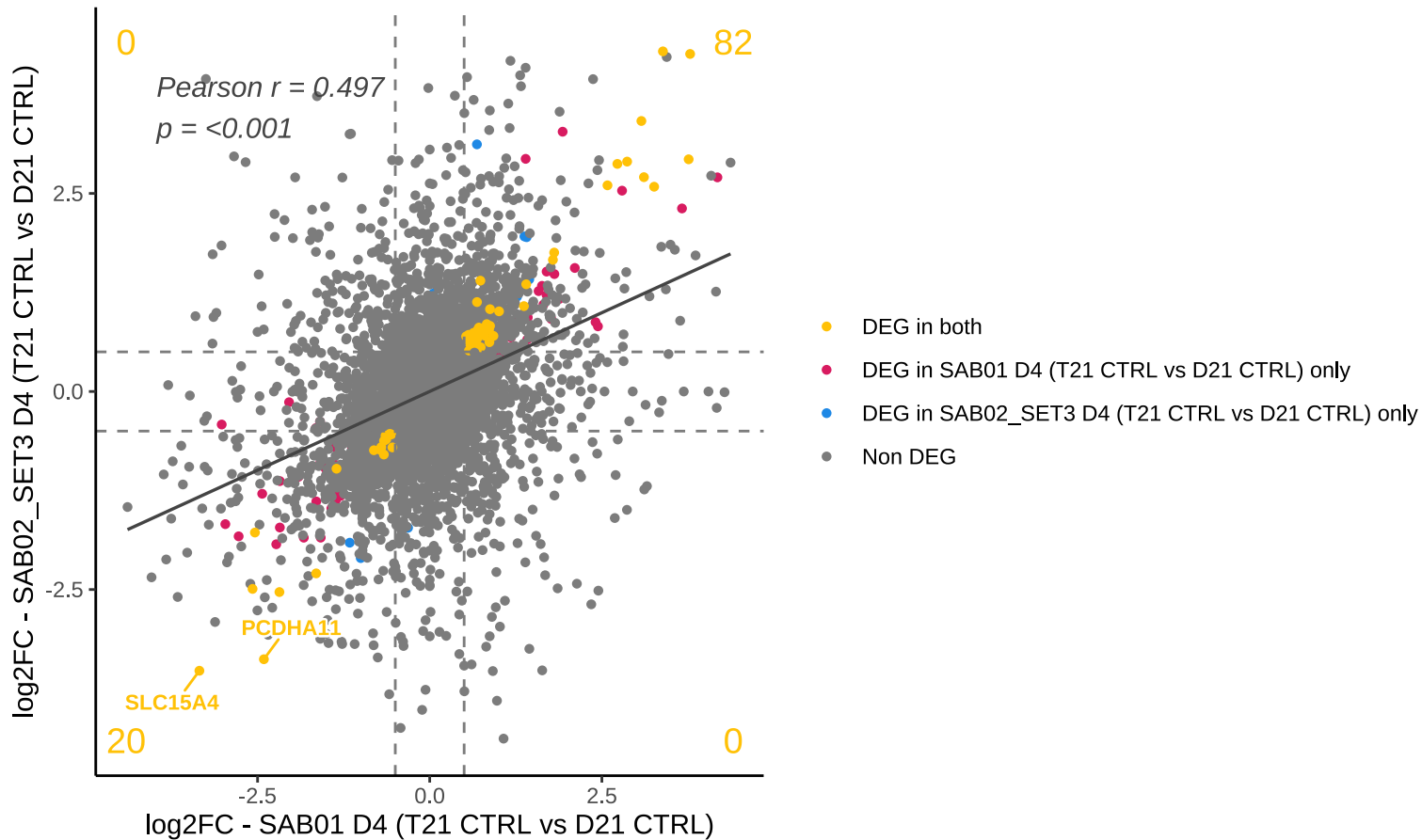
Comparison between SAB01 D4 (T21 CTRL vs D21 CTRL) and SAB02_SET3 D4 (T21 CTRL vs D21 CTRL)
