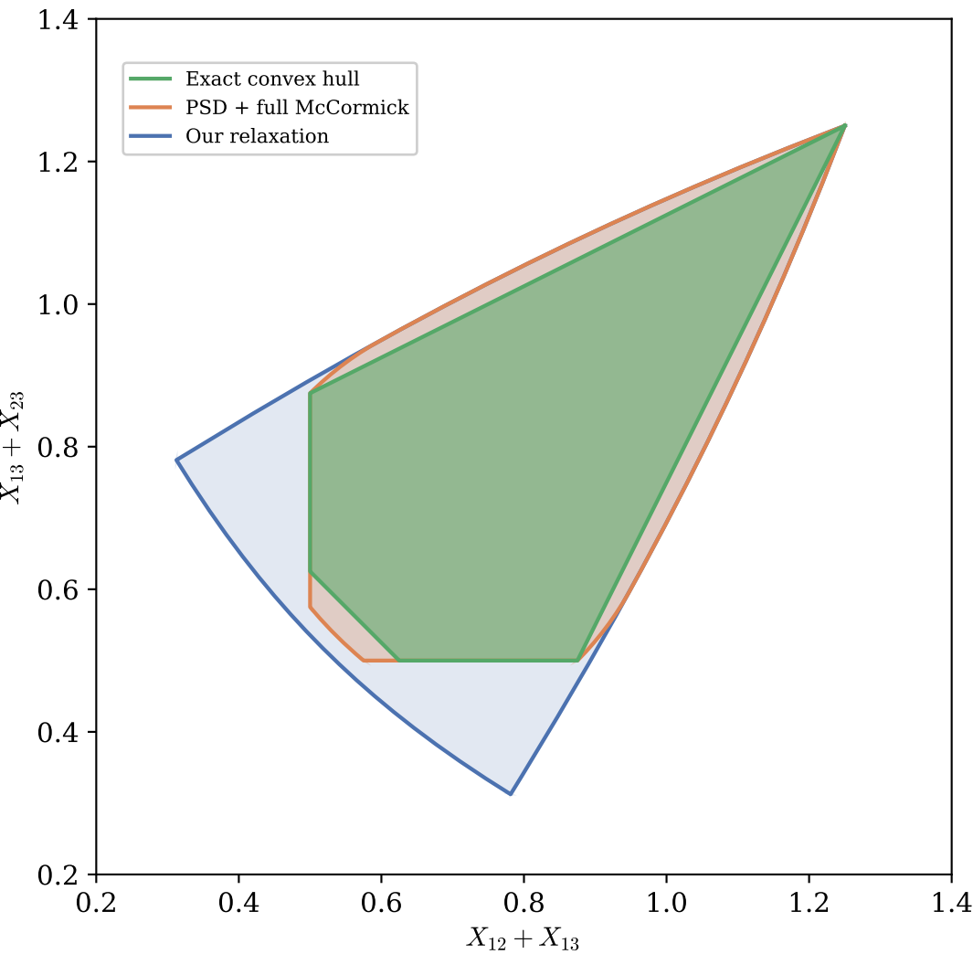
Projection to (X_{12} + X_{13}, X_{13} + X_{23})
