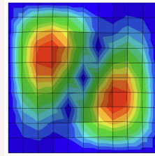
(b) Mode shape 2: \omega_{12}^h = 2.573 Hz
