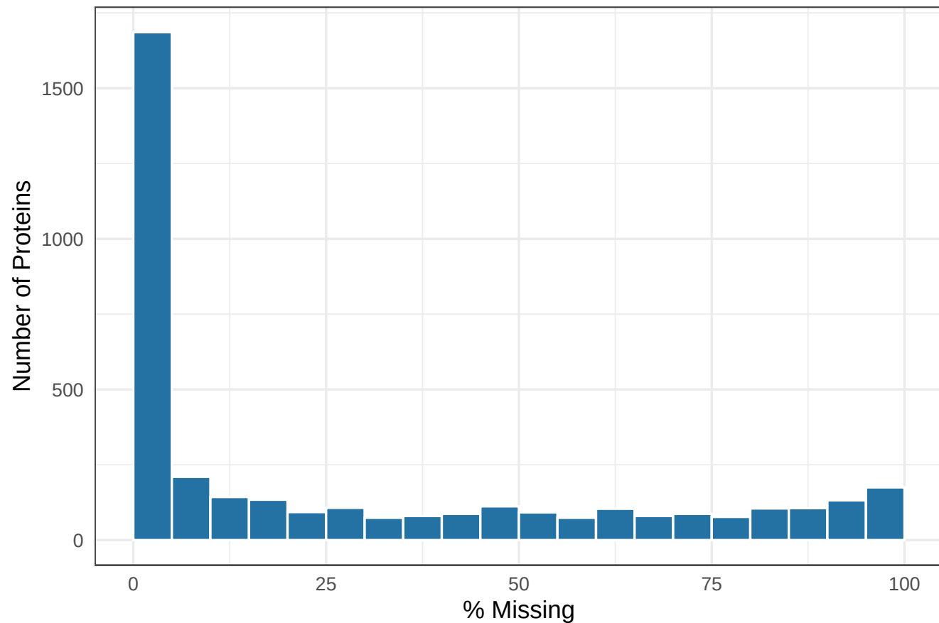
Per-Protein Missingness (Raw)
