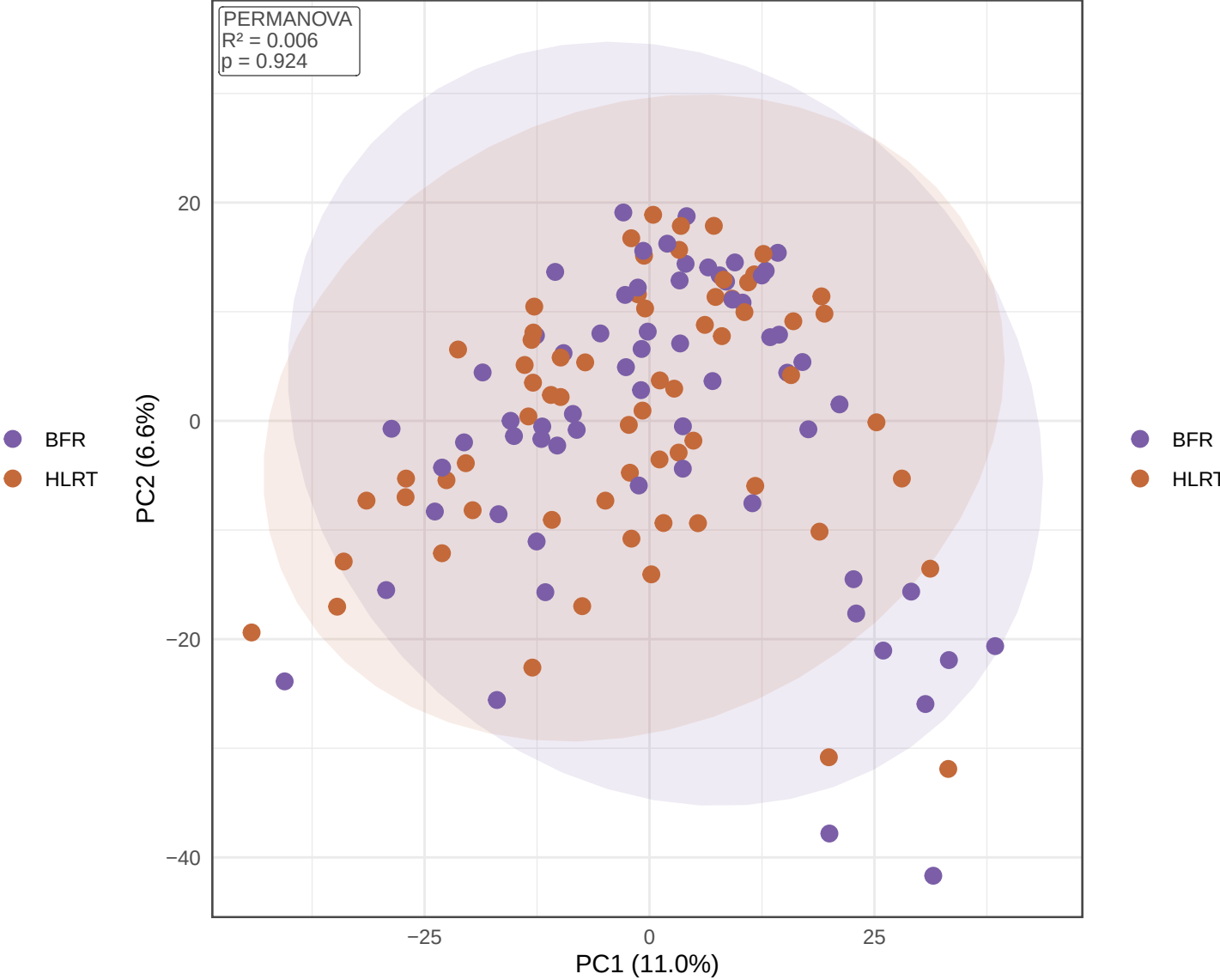
PCA – Post-Normalization
